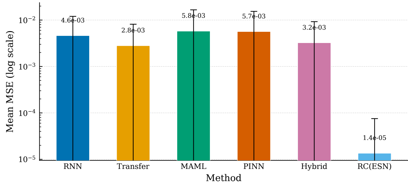
Duffing — Mean MSE Across 25 Random ICs
