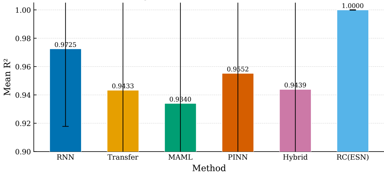
Duffing — Mean R^2 Across 25 Random ICs
