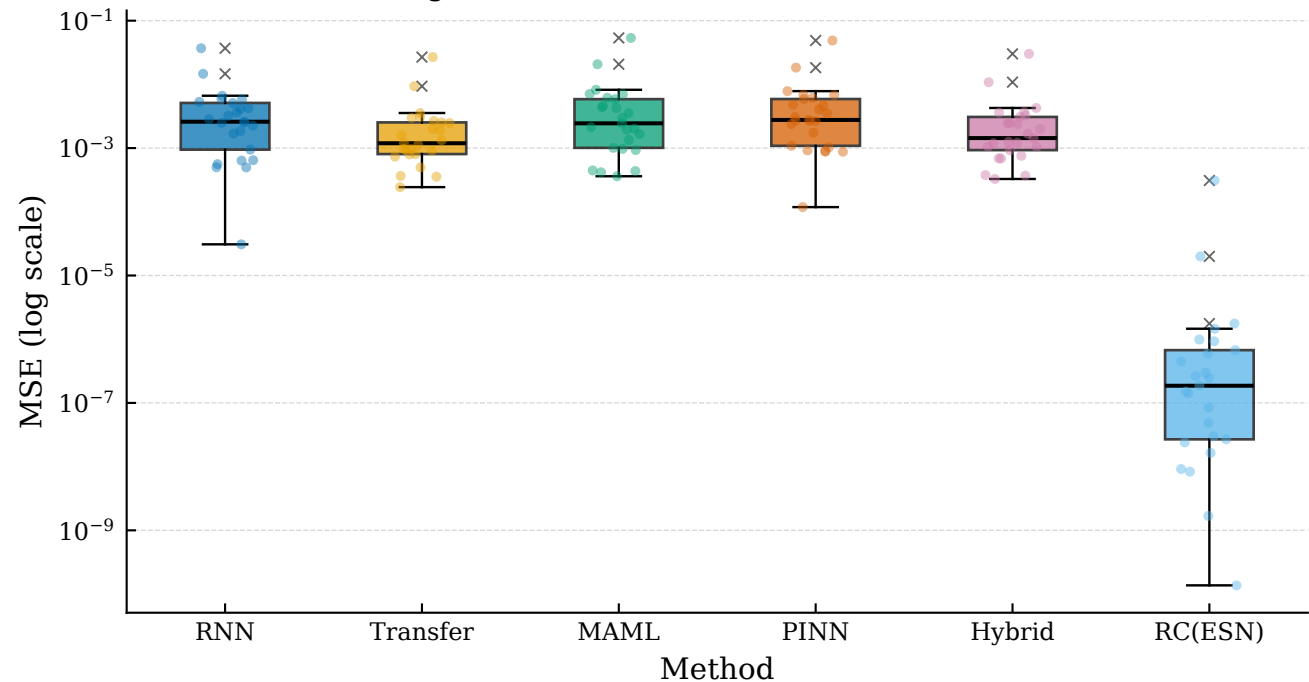
Duffing — MSE Distribution Across 25 Random ICs
