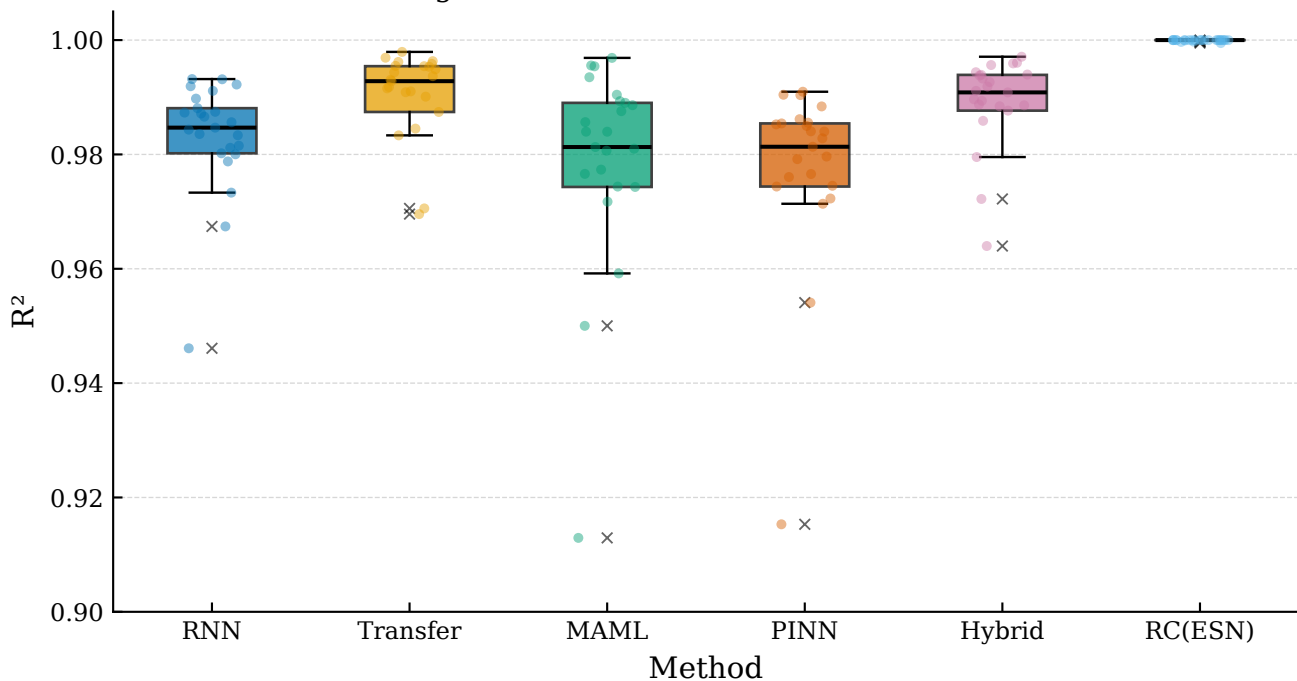
Duffing — R^2 Distribution Across 25 Random ICs
