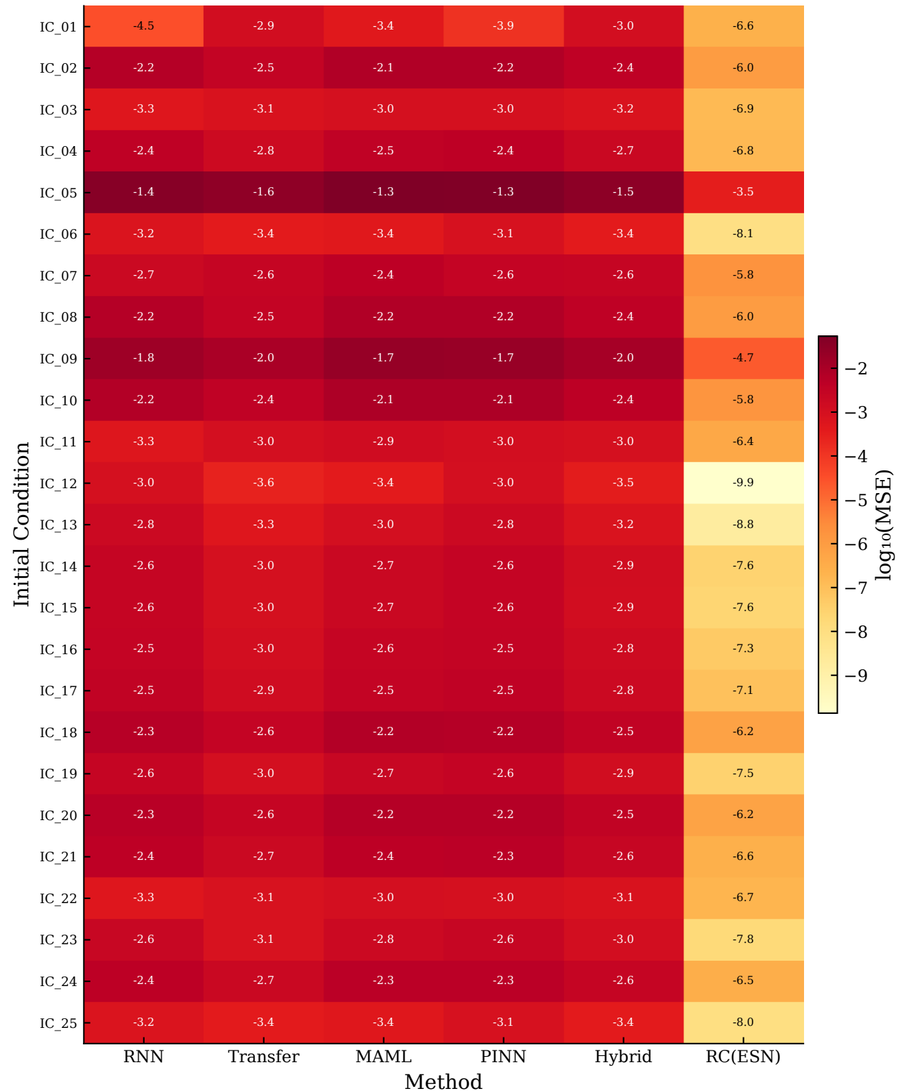
Duffing — \log_{10}(\text{MSE}) per IC and Method
