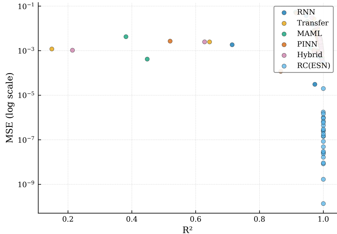
Duffing — MSE vs R^2 for All Methods and Random ICs
