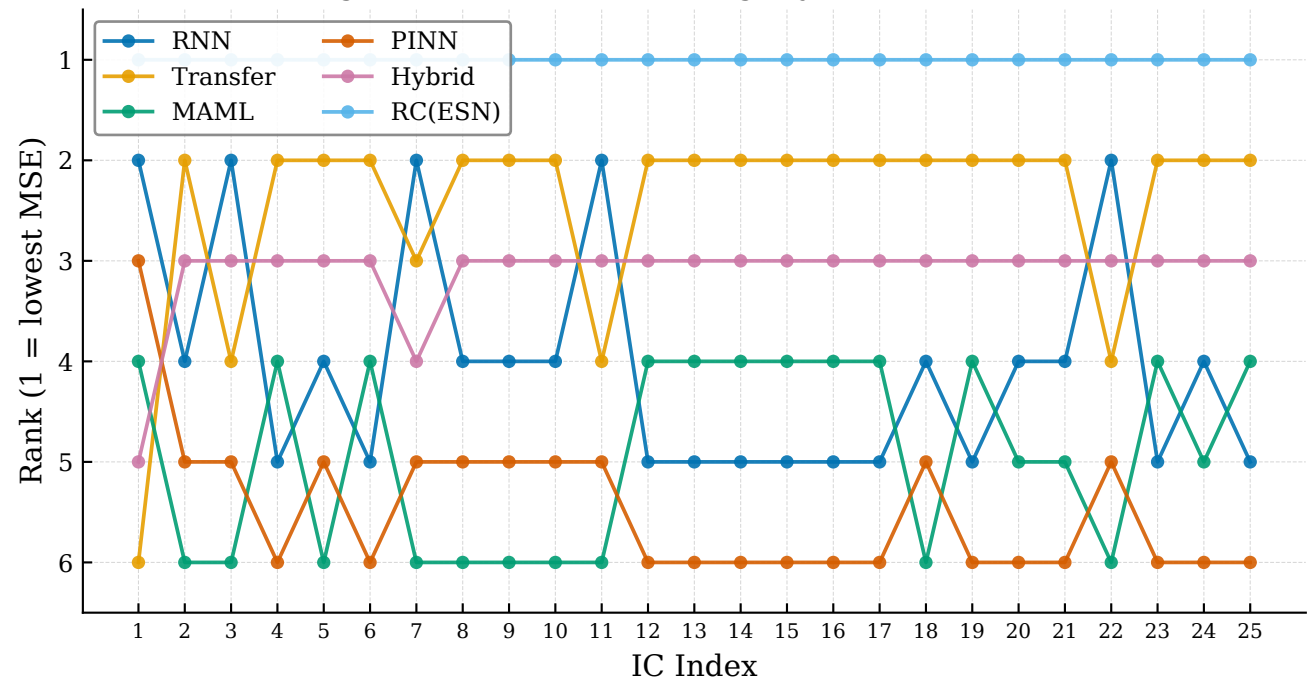
Duffing — Per-IC Method Rankings by MSE (Rank 1 = Best)
