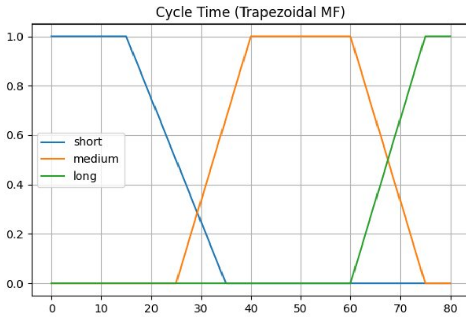
Figure 3 — Cycle Time Membership Function (Output) Trapezoidal MF · Short [0,0,15,35] · Medium [25,40,60,75] · Long [60,75,90,90]
