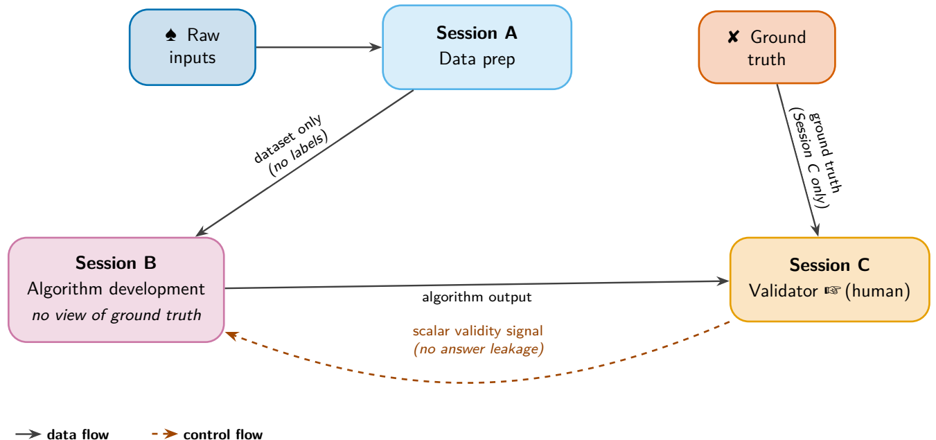
Figure 1: The session triangle. Three isolated agent sessions partition responsibility so that no single session has the privileges to cheat. Session A prepares the dataset; Session B develops the algorithm against that dataset with no view of ground truth ; Session C is the validator (currently a human) and is the only session that sees ground truth. The signal returning to Session B is restricted to a scalar validity score (dashed orange), so the algorithm-developing session cannot reverse-engineer the answer from the feedback it receives.
