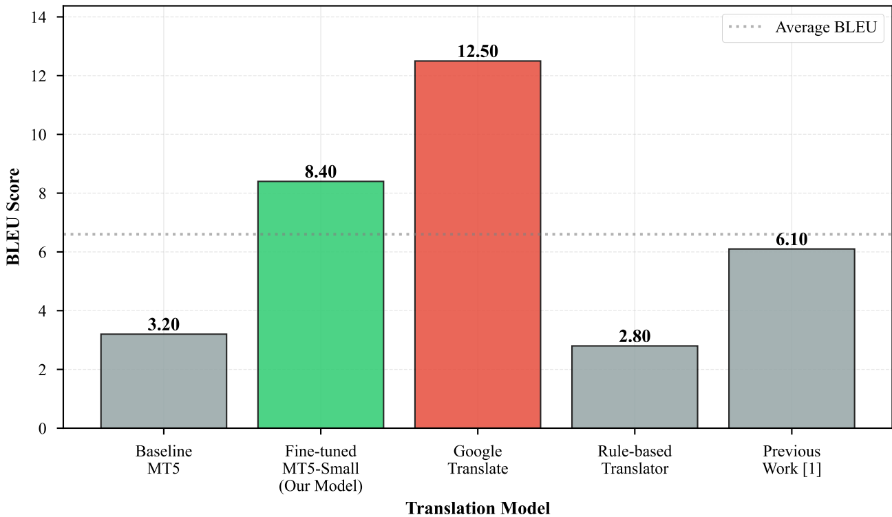
English-Tulu Translation Performance Comparison
