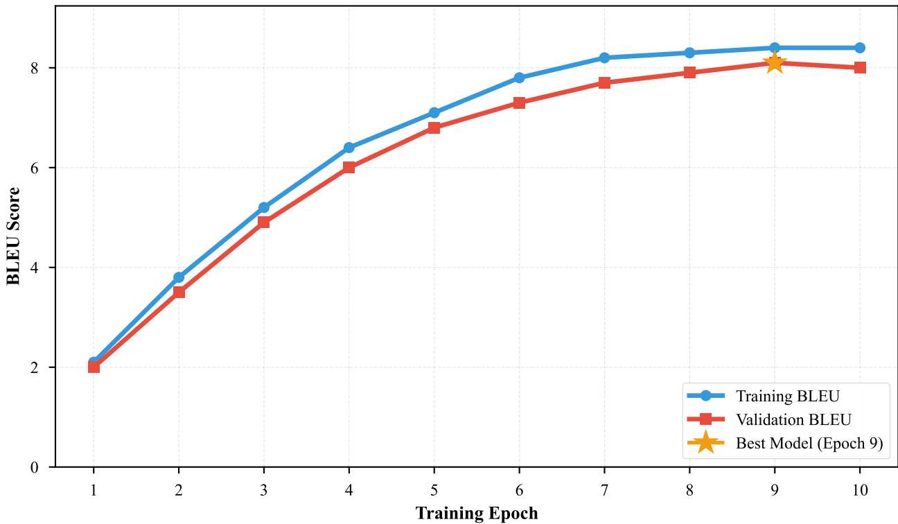
Model Training Progress on English-Tulu Translation
