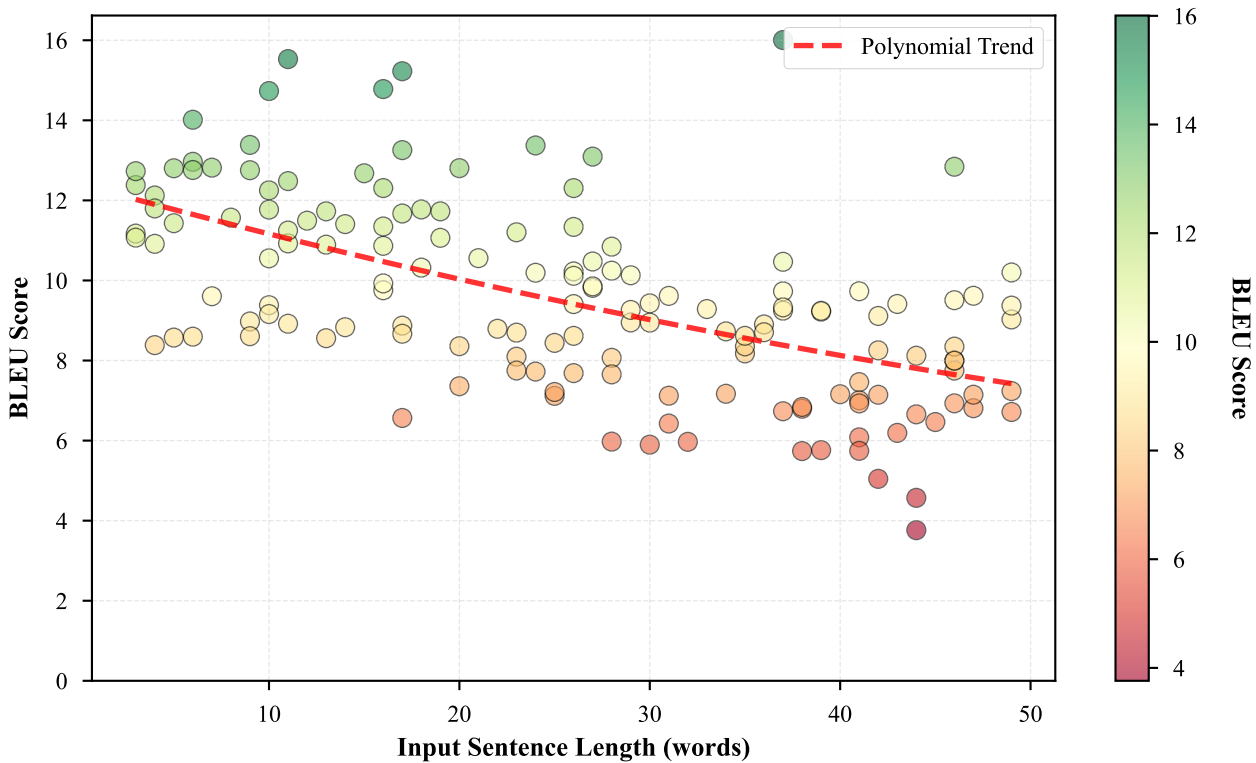
Translation Quality vs Input Length
