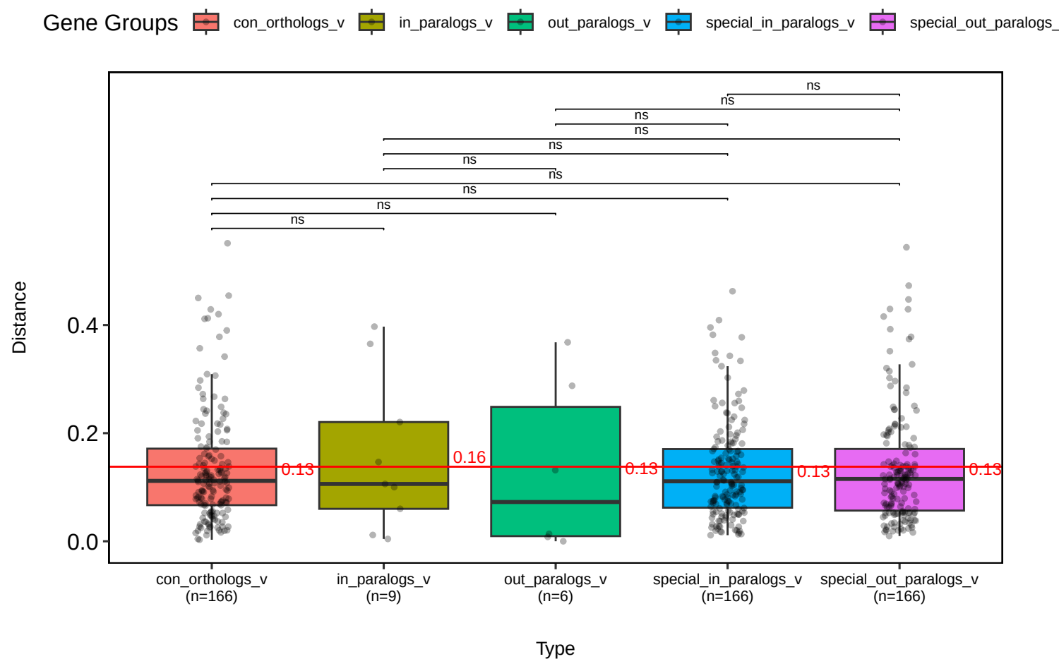
Mean Log2 Expression Distances – whole_body_dietP (wilcox.test)
