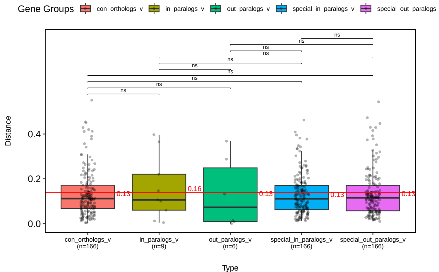
Mean Log2 Expression Distances – whole_body_dietP (t.test)
