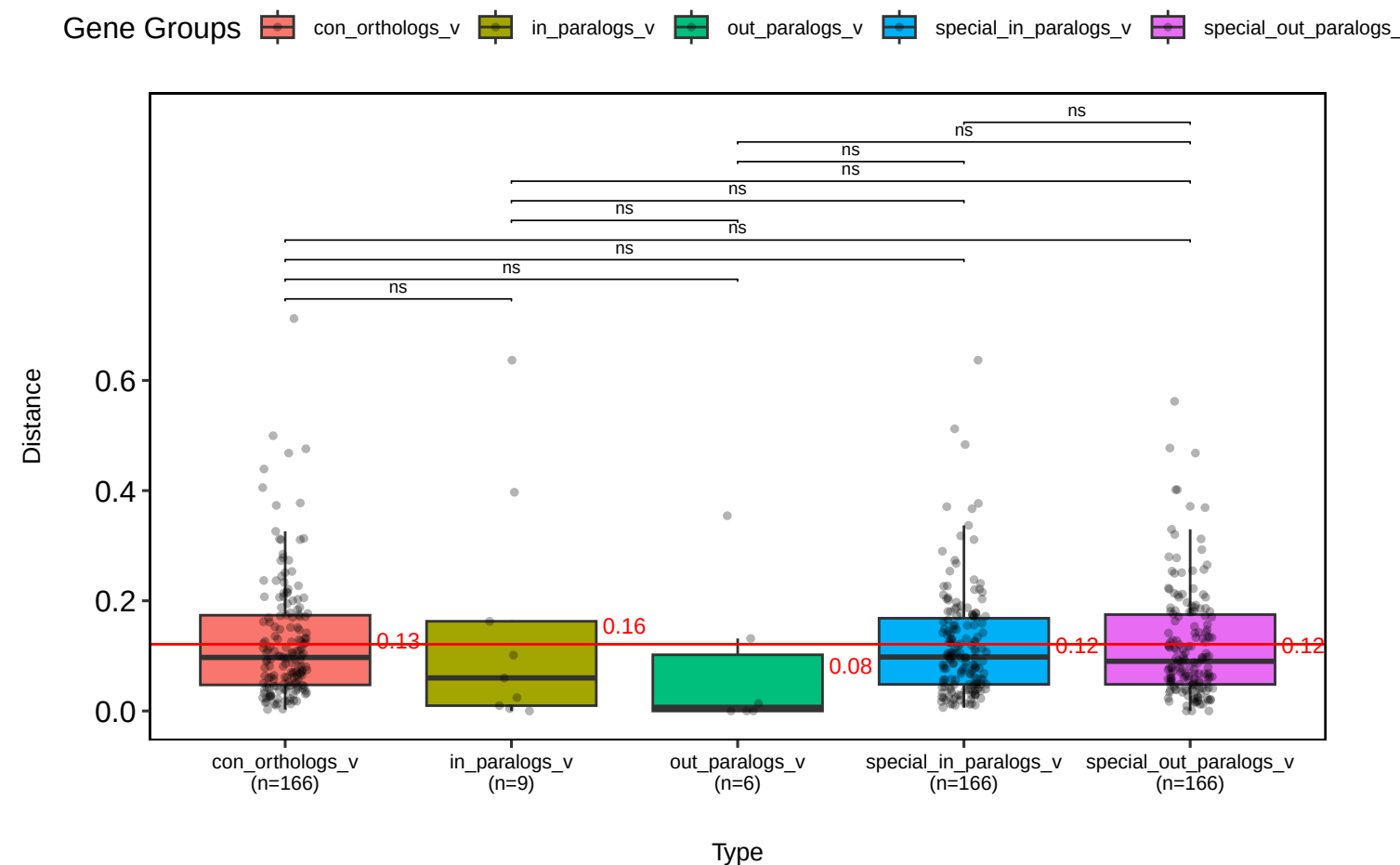
Median Log2 Expression Distances – whole_body_dietP (t.test)
