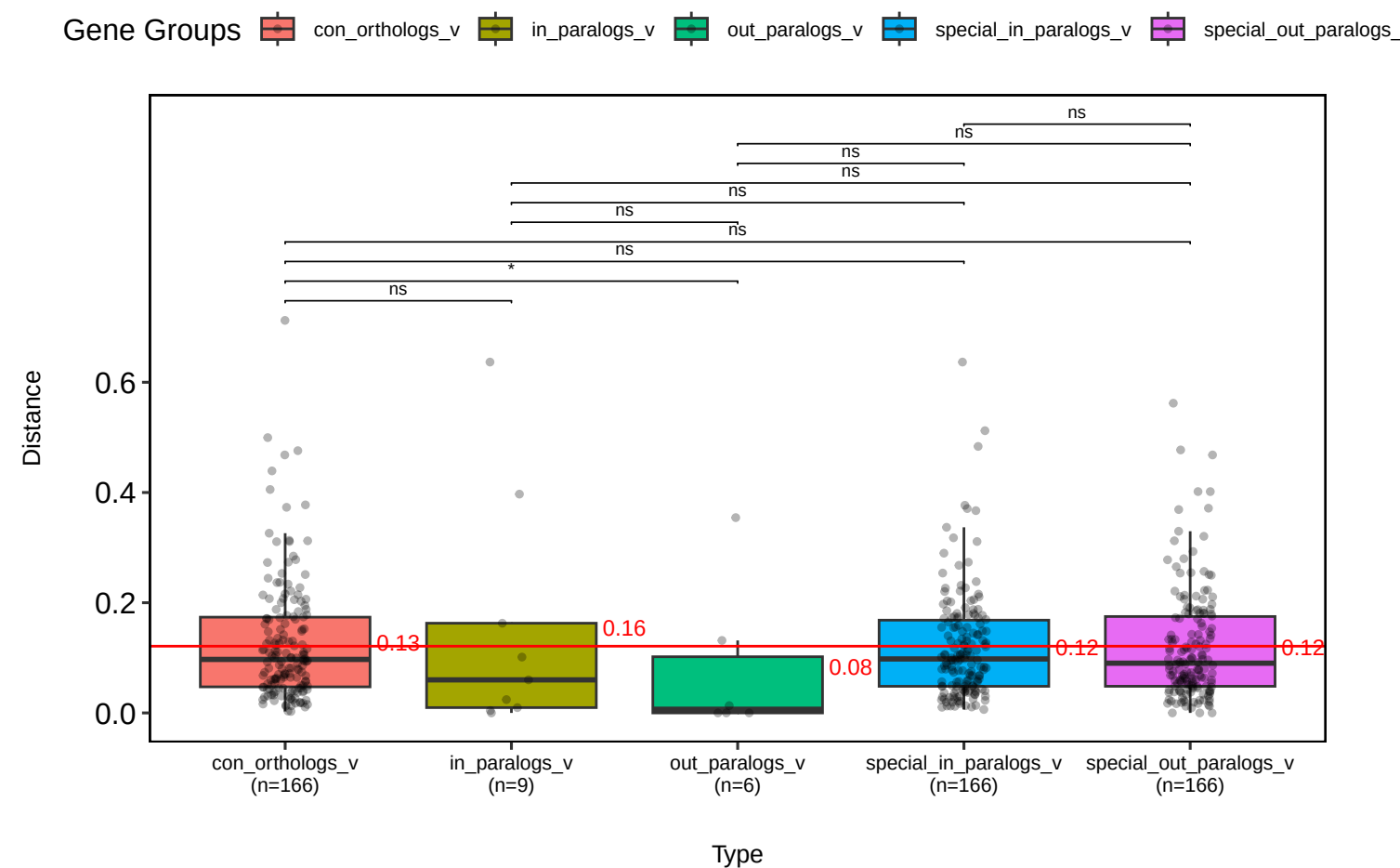
Median Log2 Expression Distances – whole_body_dietP (wilcox.test)
