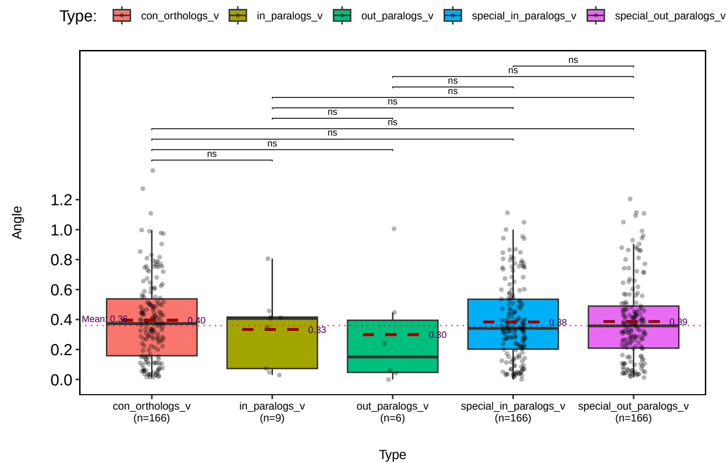
Mean Expression Angle (wilcox.test)
