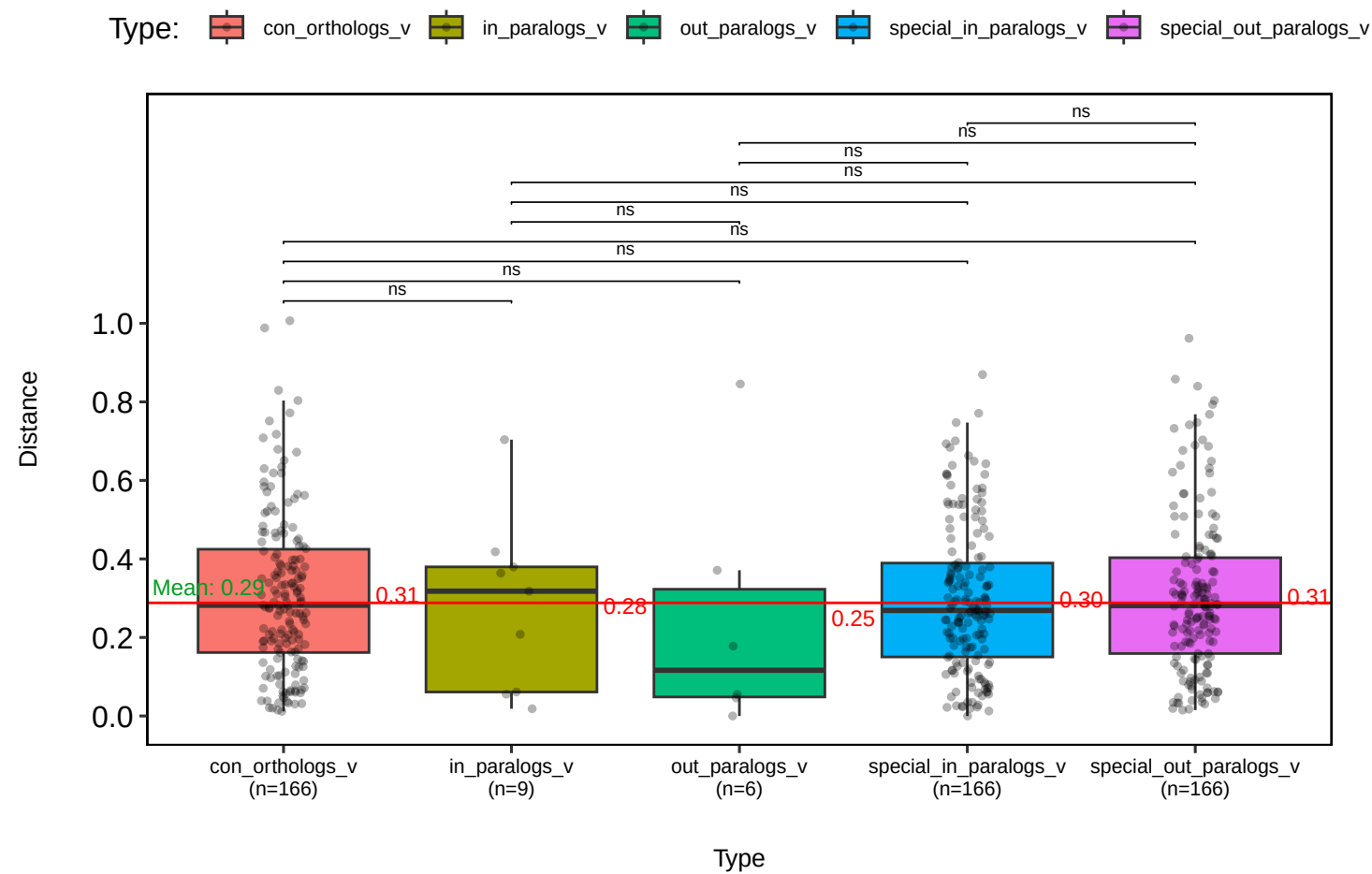
Mean Expression Distance (t.test)
