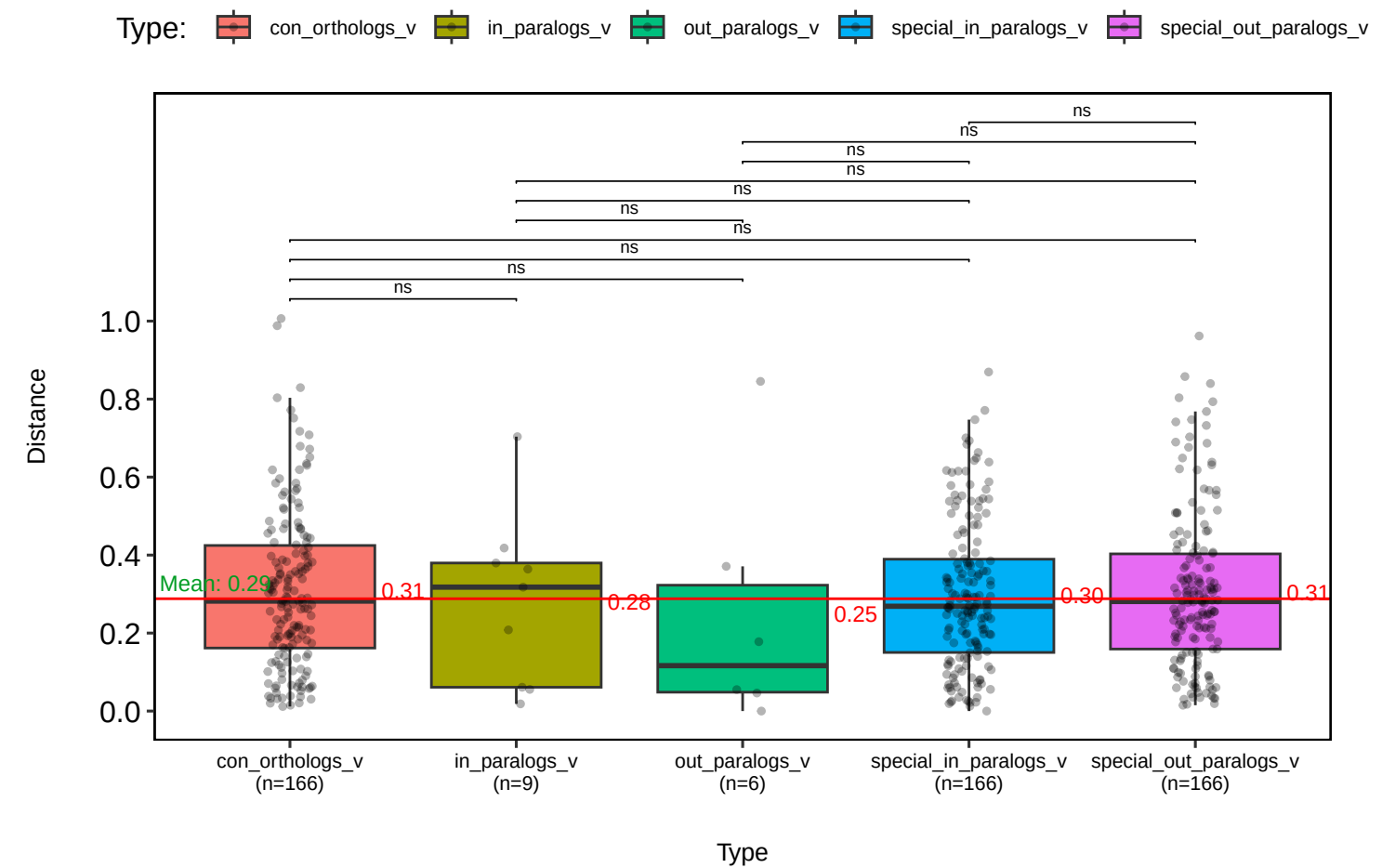
Mean Expression Distance (wilcox.test)
