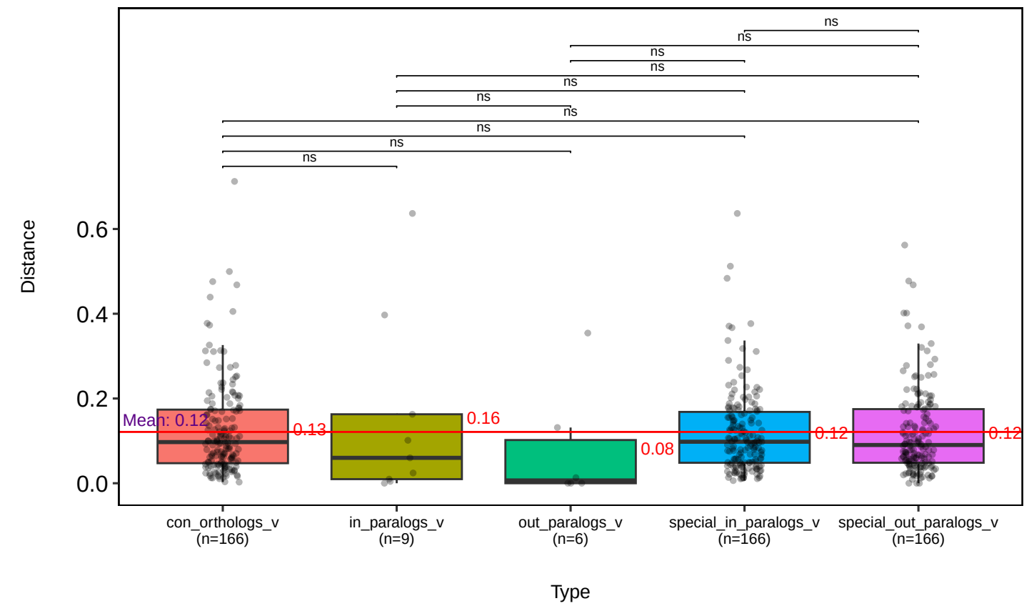
Median Log2 Expression Distances – whole_body_dietP (wilcox.test)
