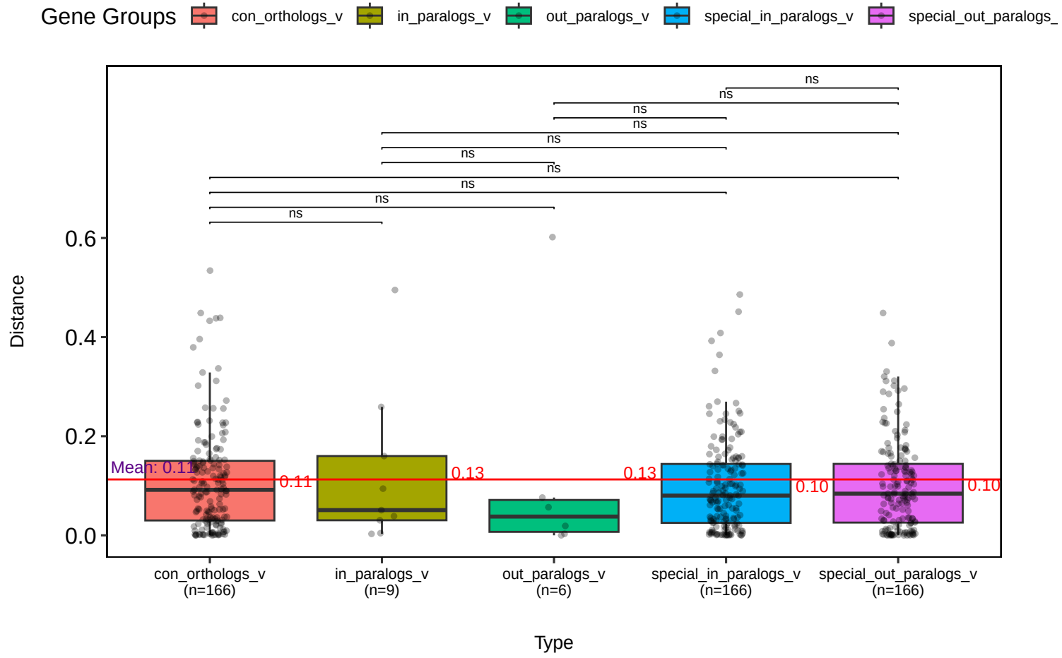
Mean Expression Distances – muscle_dietP (wilcox.test)
