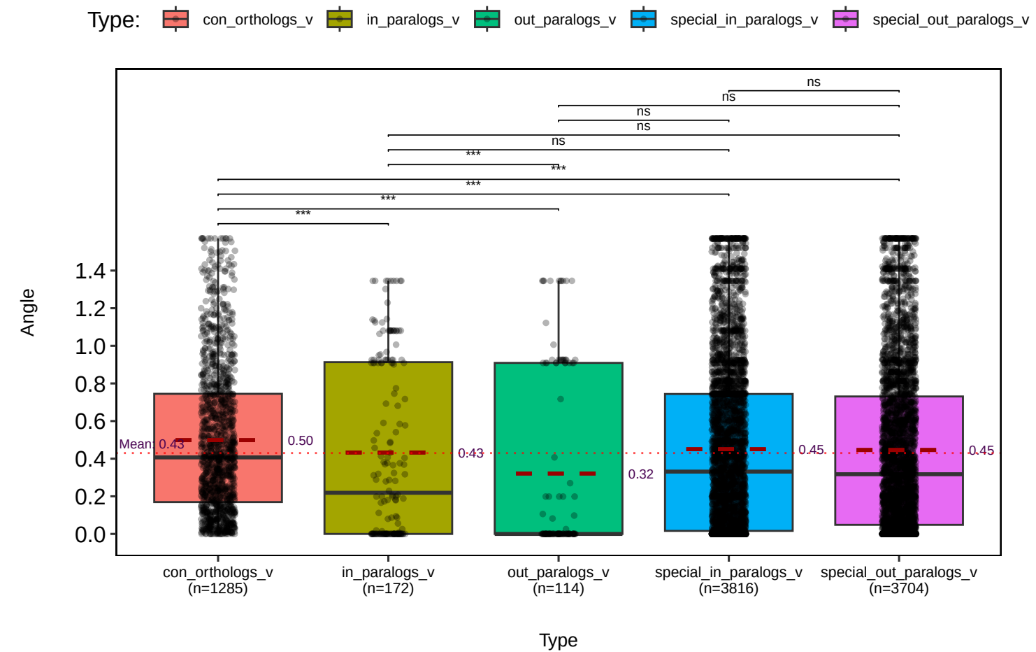
Log2 Expression Angle (wilcox.test)
