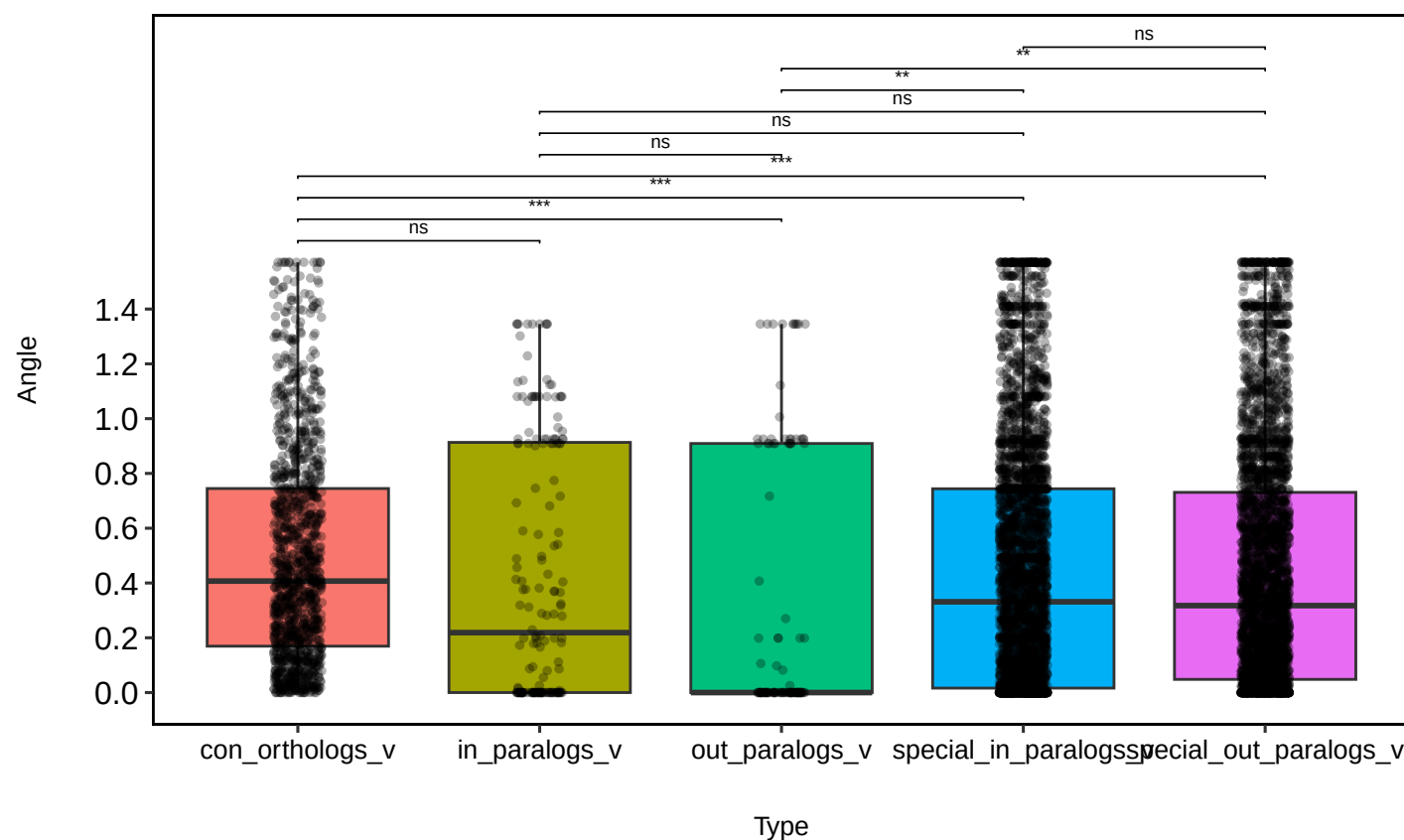
Log2 Expression Angles (t.test)
