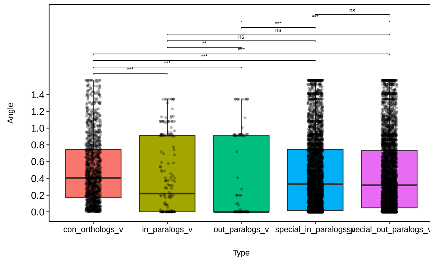
Log2 Expression Angles (wilcox.test)
