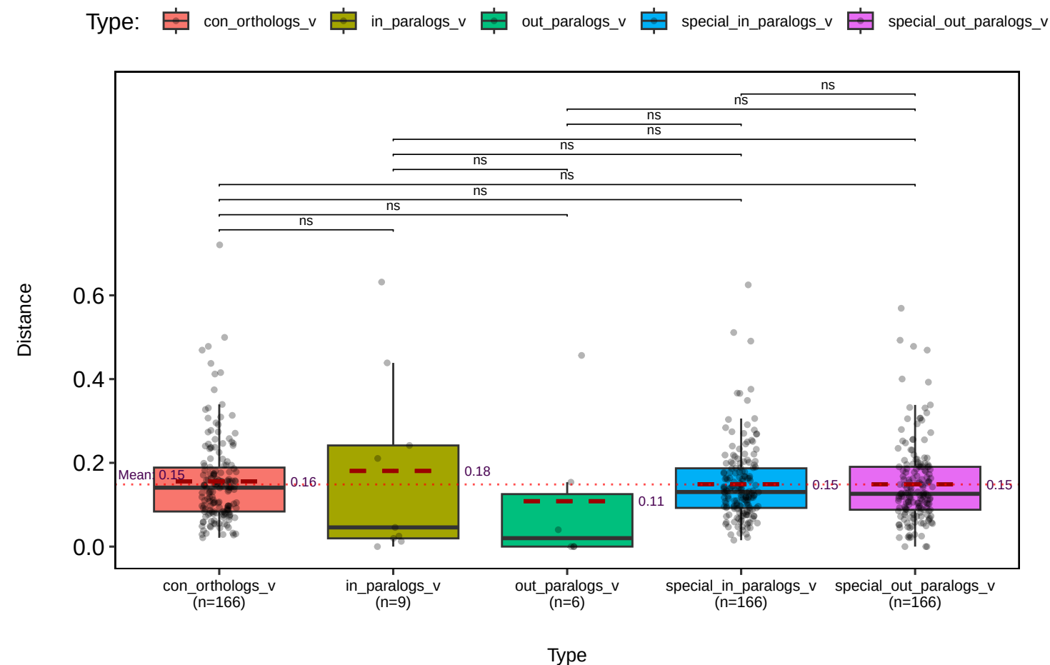
Median Expression Distances – whole_body_dietP (wilcox.test)
