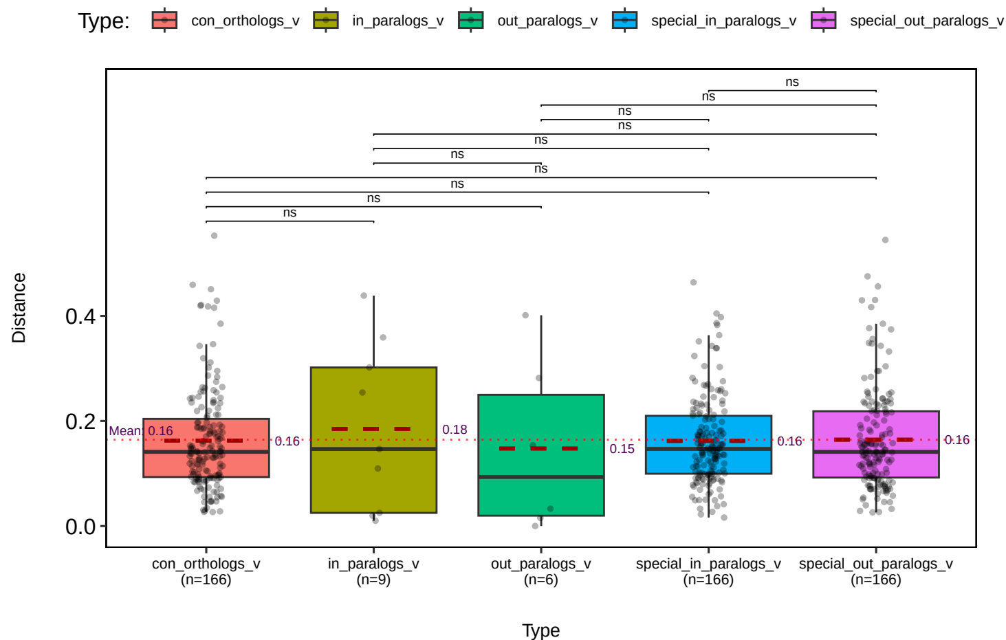
Mean Expression Distances – whole_body_dietP (wilcox.test)
