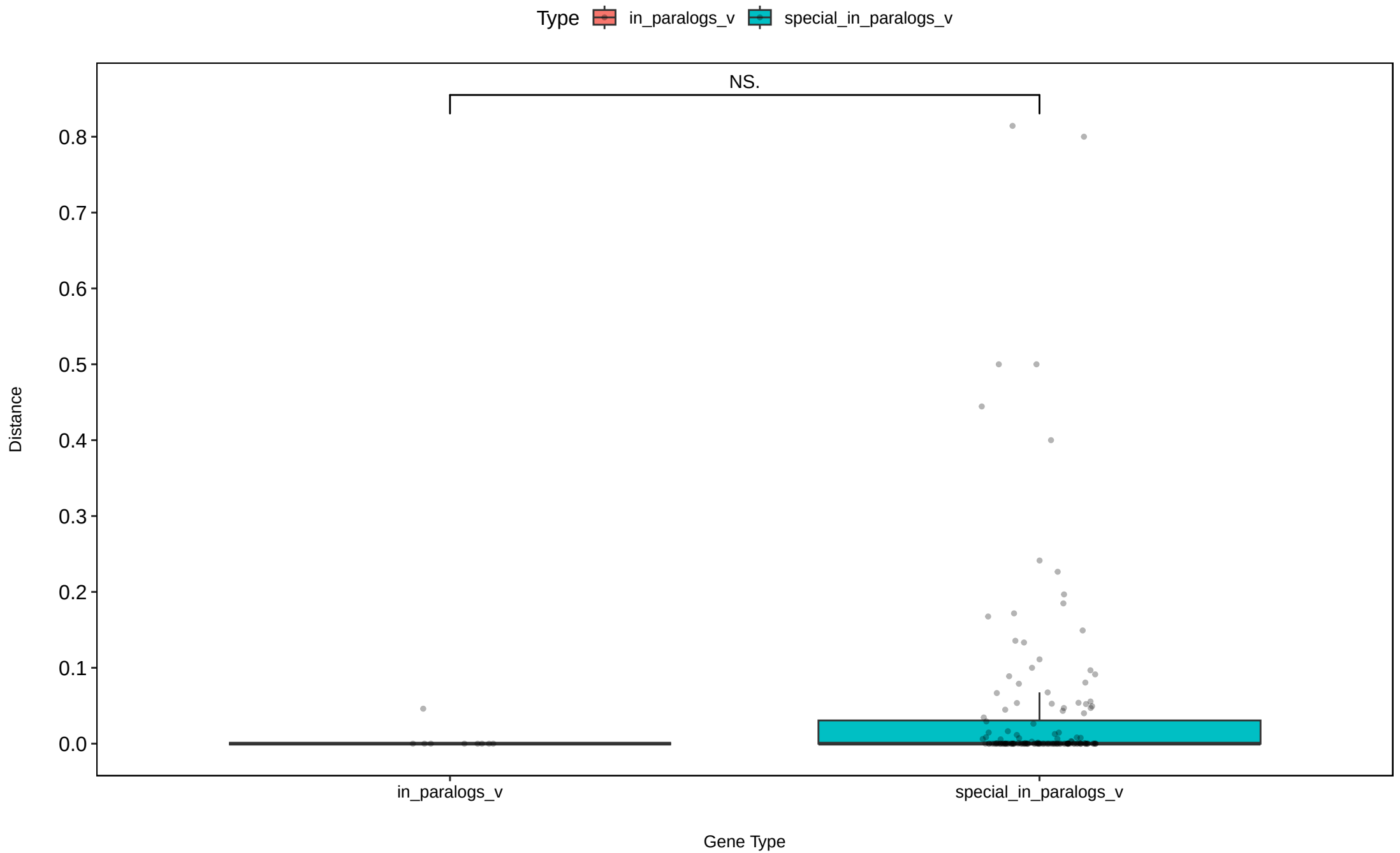
Median Expression Distances – mE_mRNA_A_MateF_4d_ovary
