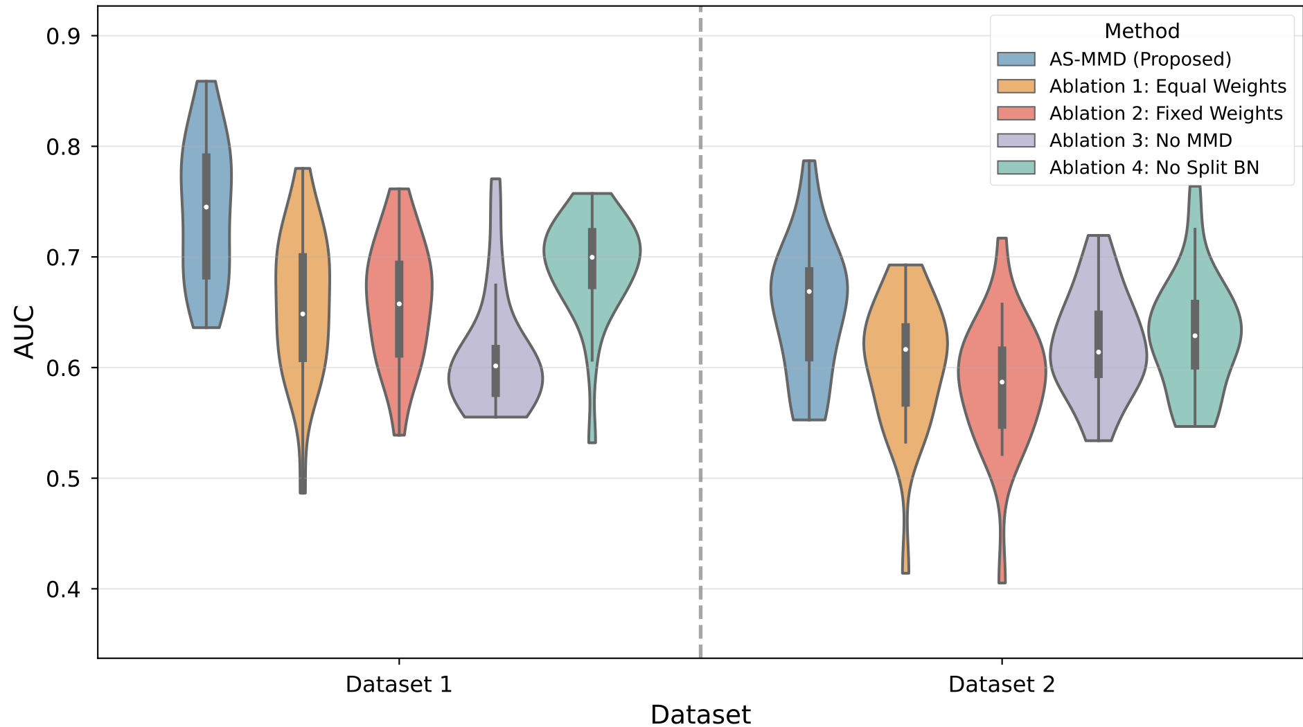
AUC Distribution: AS-MMD vs Ablation Studies
