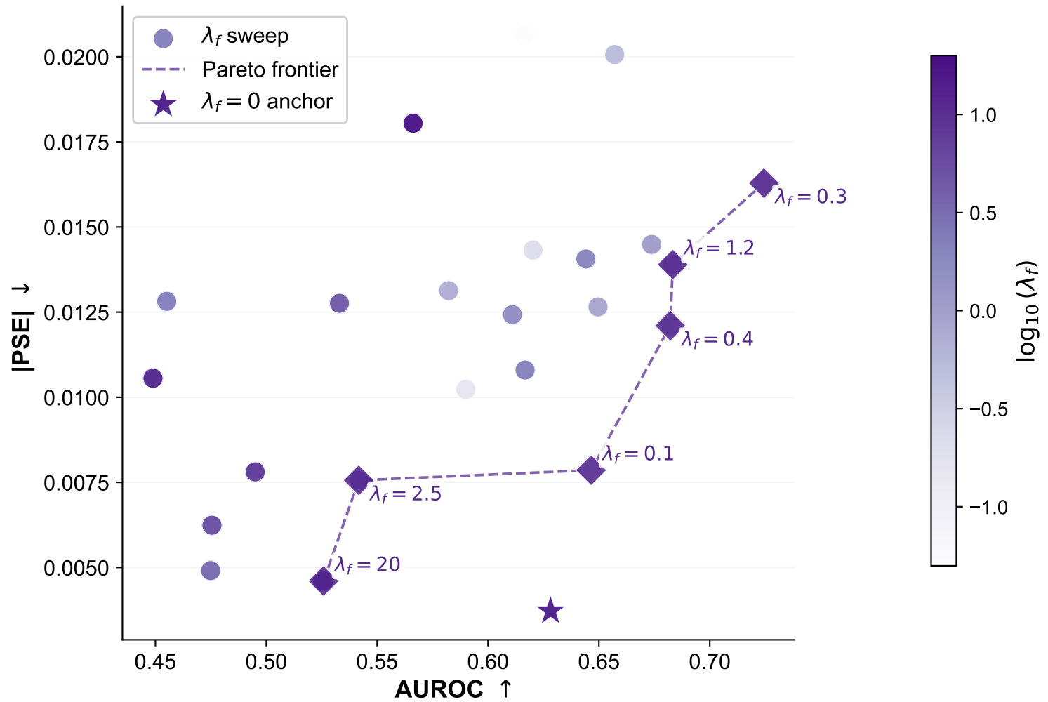
AUROC vs |PSE|
