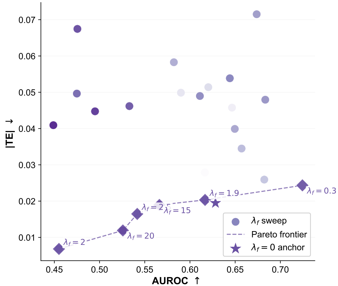
AUROC vs |TE|
