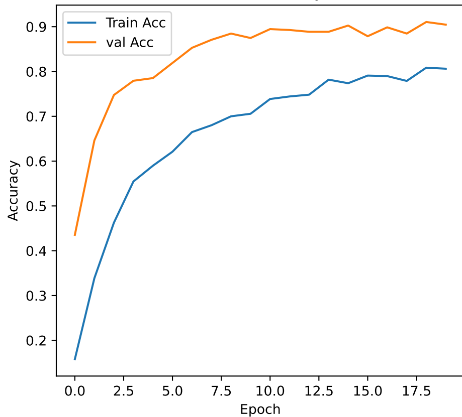
Model Accuracy
