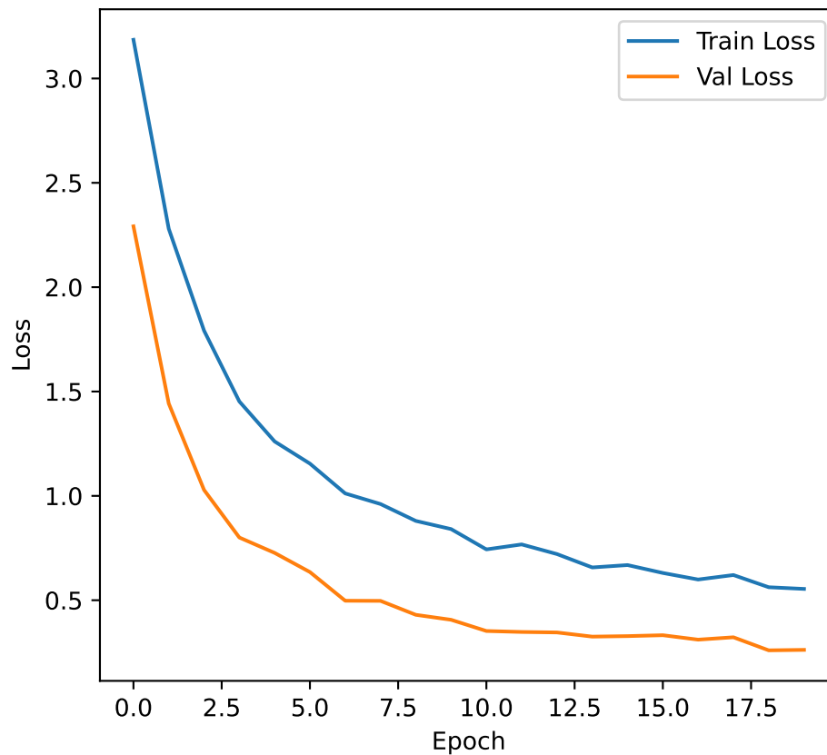
model Loss
