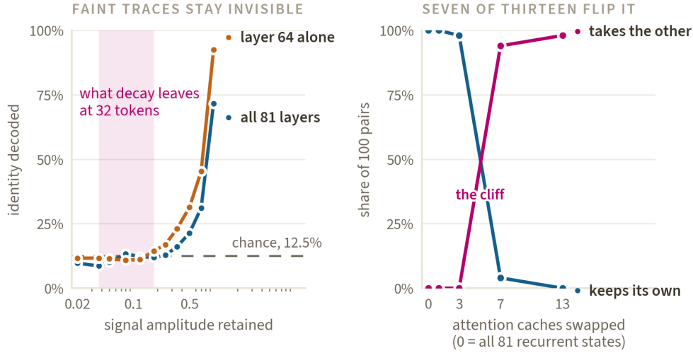
Figure 3: Left: the probe’s detection floor. The shaded band is what decay leaves of a stored trace after 32 tokens; both probes are at chance throughout it, so a visible reading there cannot be retained content. Right: how many attention caches must be exchanged before the answer follows the other image; the leftmost point is the full recurrent swap, with no effect.
