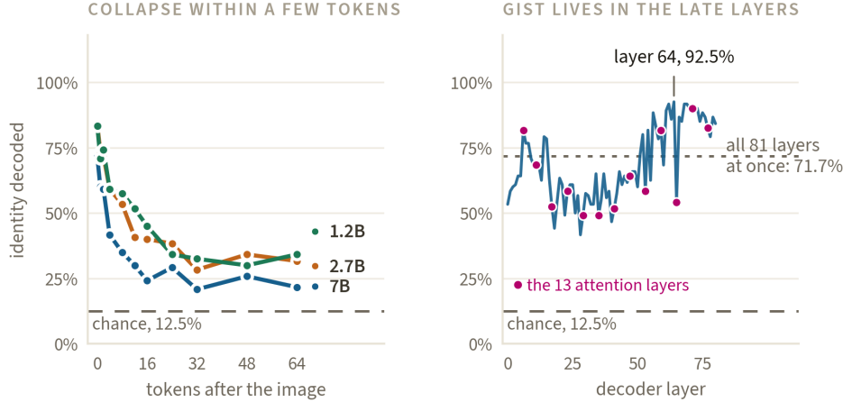
Figure 1: Left: identity decoded from the recurrent state against distance, at three scales, 120 trials per point; the pre-image control reads exactly 12.5%. Right: identity decoded from each layer’s state at the instant of writing; red marks the 13 layers that also carry attention.
