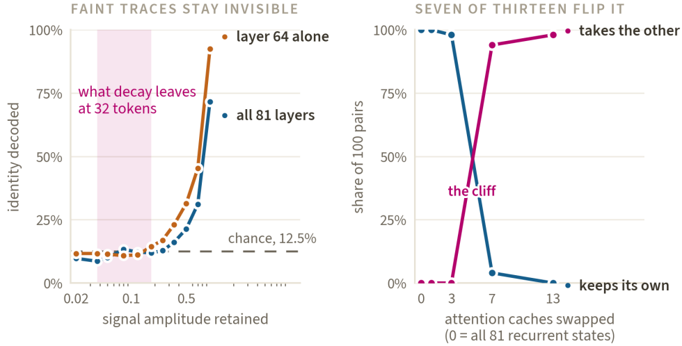
Figure 3: Left: the probe's detection floor. The shaded band is what decay leaves of a stored trace after 32 tokens; both probes are at chance throughout it, so a visible reading there cannot be retained content. Right: how many attention caches must be exchanged before the answer follows the other image; the leftmost point is the full recurrent swap, with no effect.
