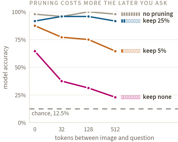
Figure 5: Model accuracy under visual key-value eviction, against how far the question sits from the image, n = 48 per point. The unpruned line is flat, so distance alone costs nothing. Keeping a quarter of the entries is also flat. Below that the lines fan out: the cost of pruning grows with distance only once the recurrent channel has stopped relaying the picture.
