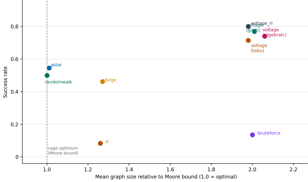
Figure 9: Cage construction: coverage versus graph size relative to the Moore bound.
