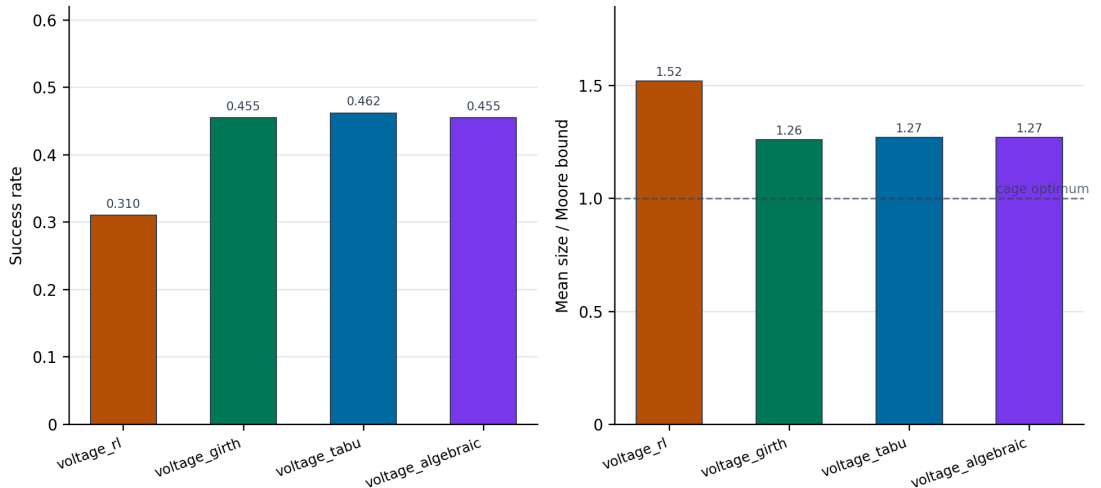
Figure 10: Forge by producer: success rate and mean graph size vs. the Moore bound.
