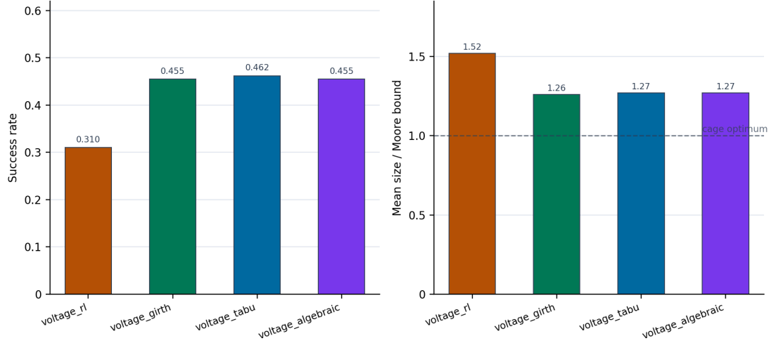
Figure 8: Forge by producer: success rate (left) and mean graph size relative to the Moore bound (right, dashed line at the cage optimum). The three non-RL producers tie and beat the reinforcement-learning producer on both.
