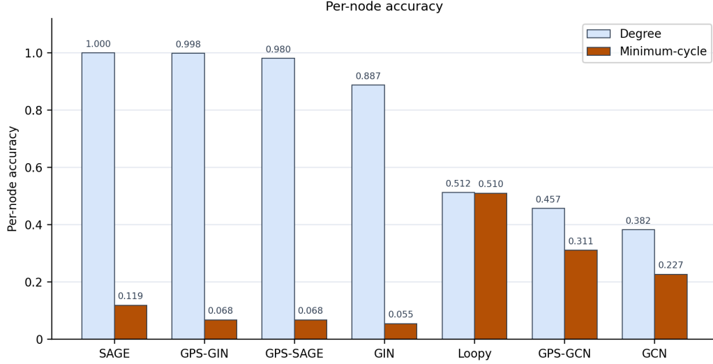
Figure 6: Per-node accuracy of the best model of each architecture on degree prediction versus minimum-cycle prediction.
