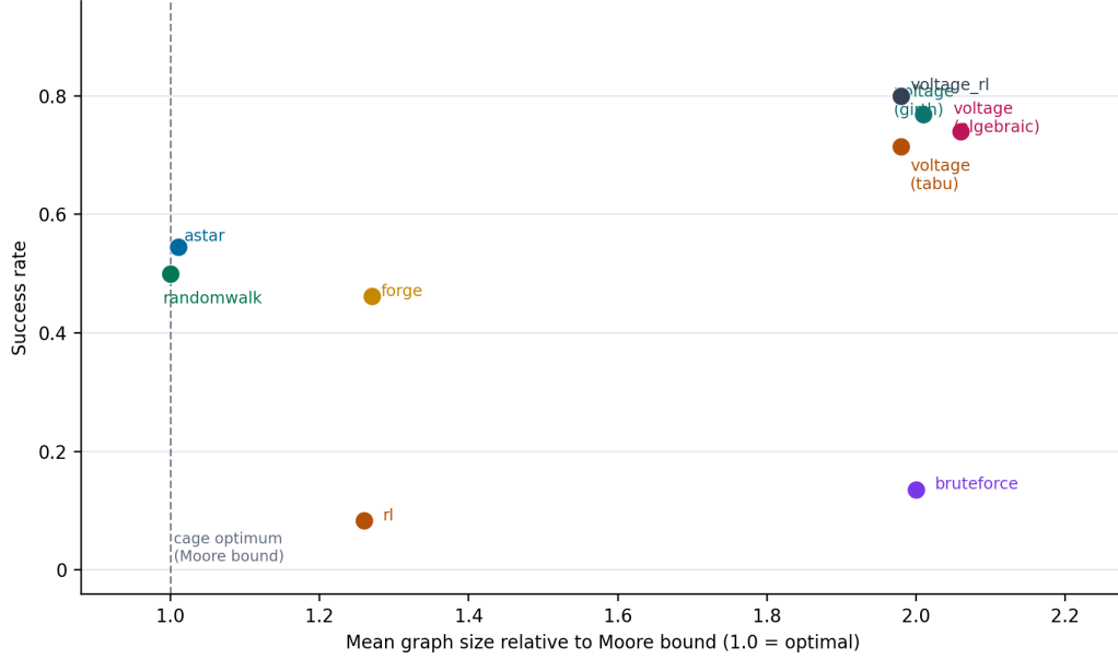
Figure 7: Coverage versus optimality. Each method is placed by its mean graph size relative to the Moore bound (horizontal, 1.0 is cage-optimal) and its success rate (vertical). Classical searches are optimal in size but low in coverage; the voltage family is the opposite; forge sits between them.
