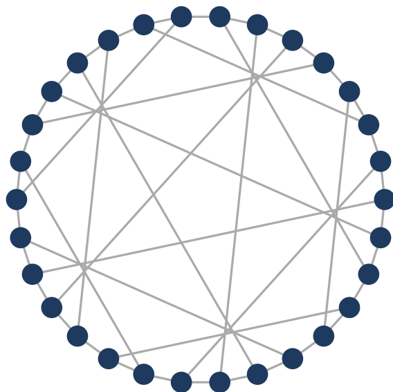
Tutte-Coxeter — (3,8)
