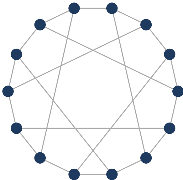
Heawood — (3,6)
