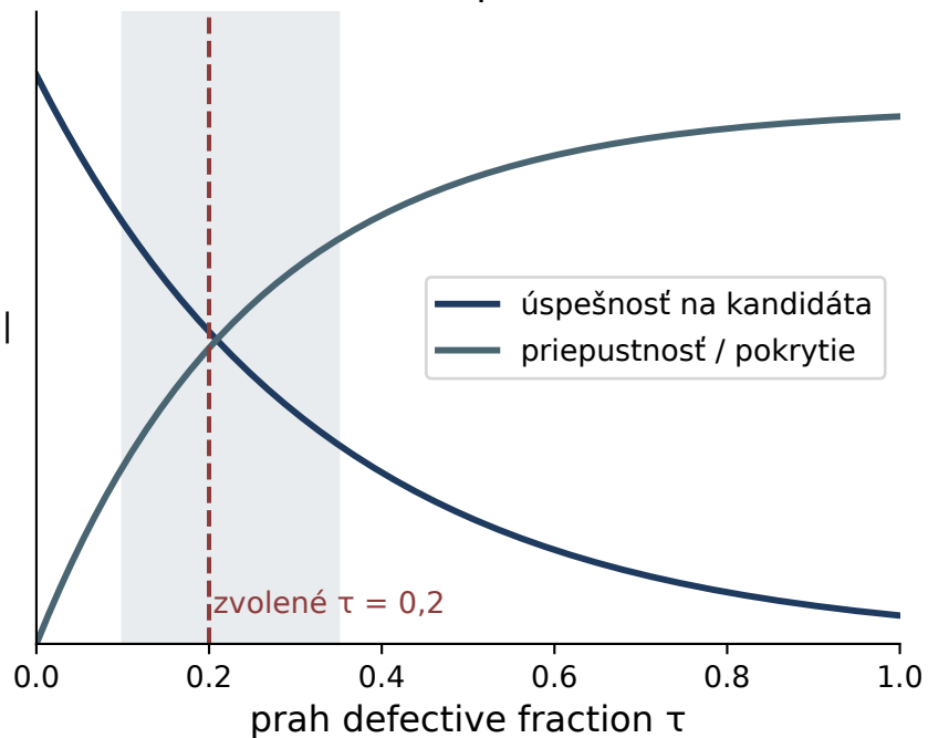
Ladenie prahu \tau
