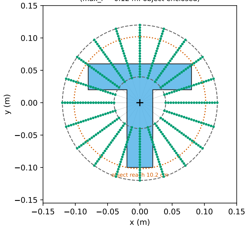
(b) proposed ( \max_r = 0.12 m: object enclosed)
