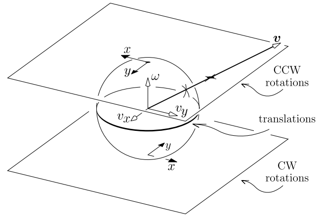
Fig. 3. The mapping \text{COR}() from velocity directions on the unit sphere to rotation centers in the slider frame \mathcal{F}_S .
