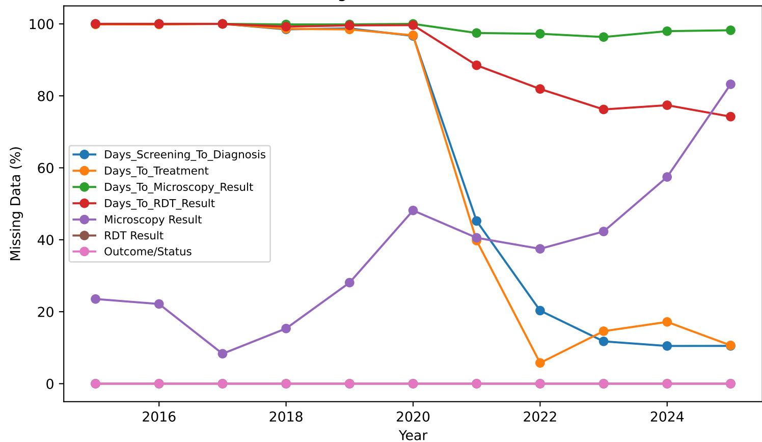
Missing Data Trends Over Time
