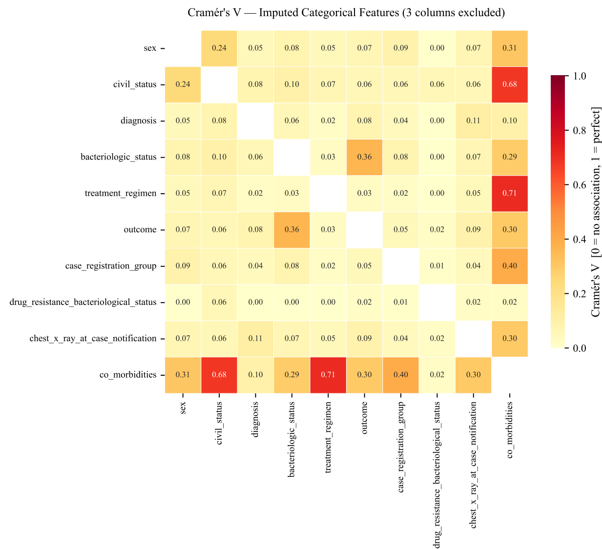
Figure 18 Cramér’s V Correlation Matrix of Imputed Categorical Variables
