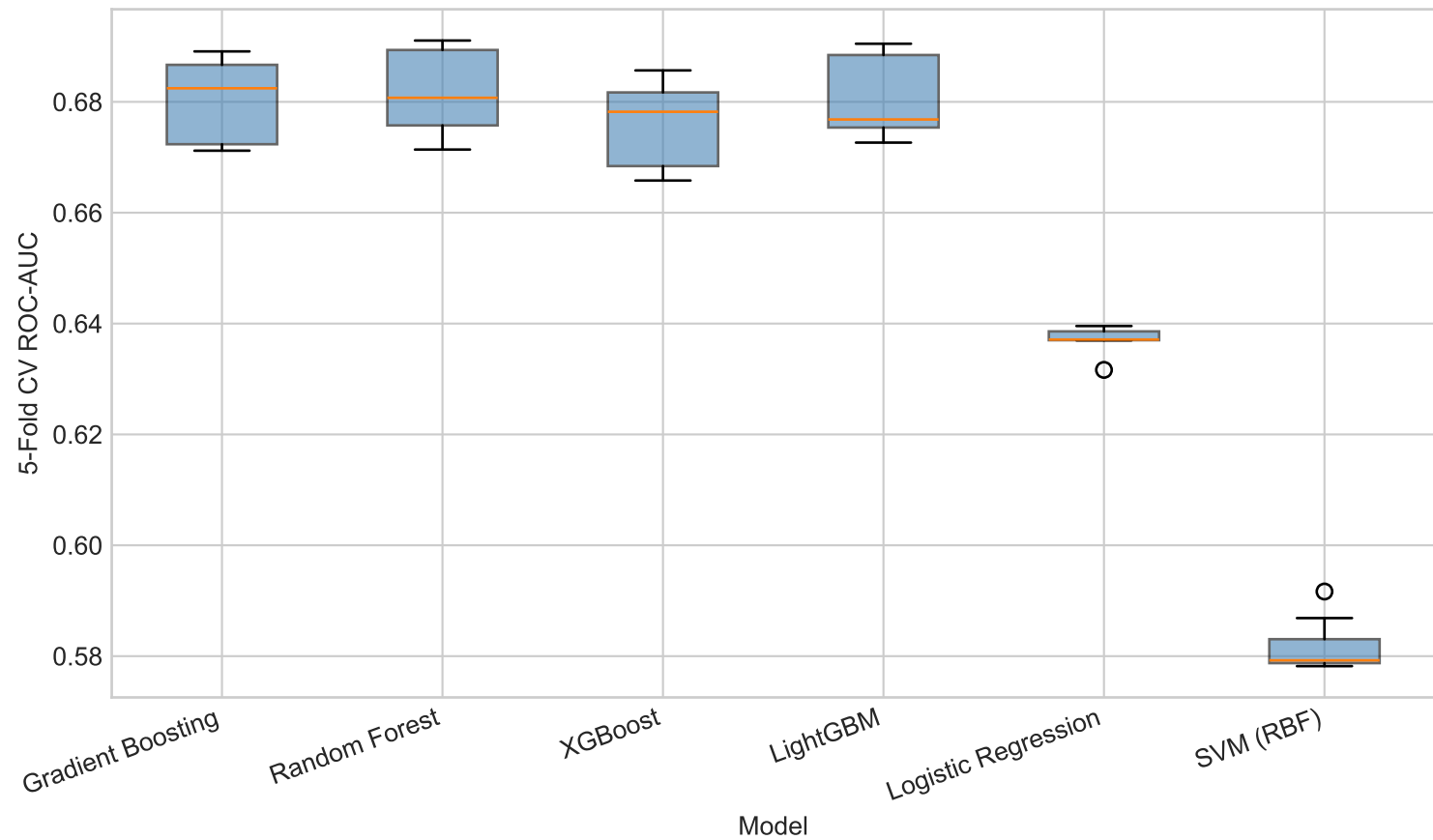
Cross-Validation ROC-AUC Distribution per Model
