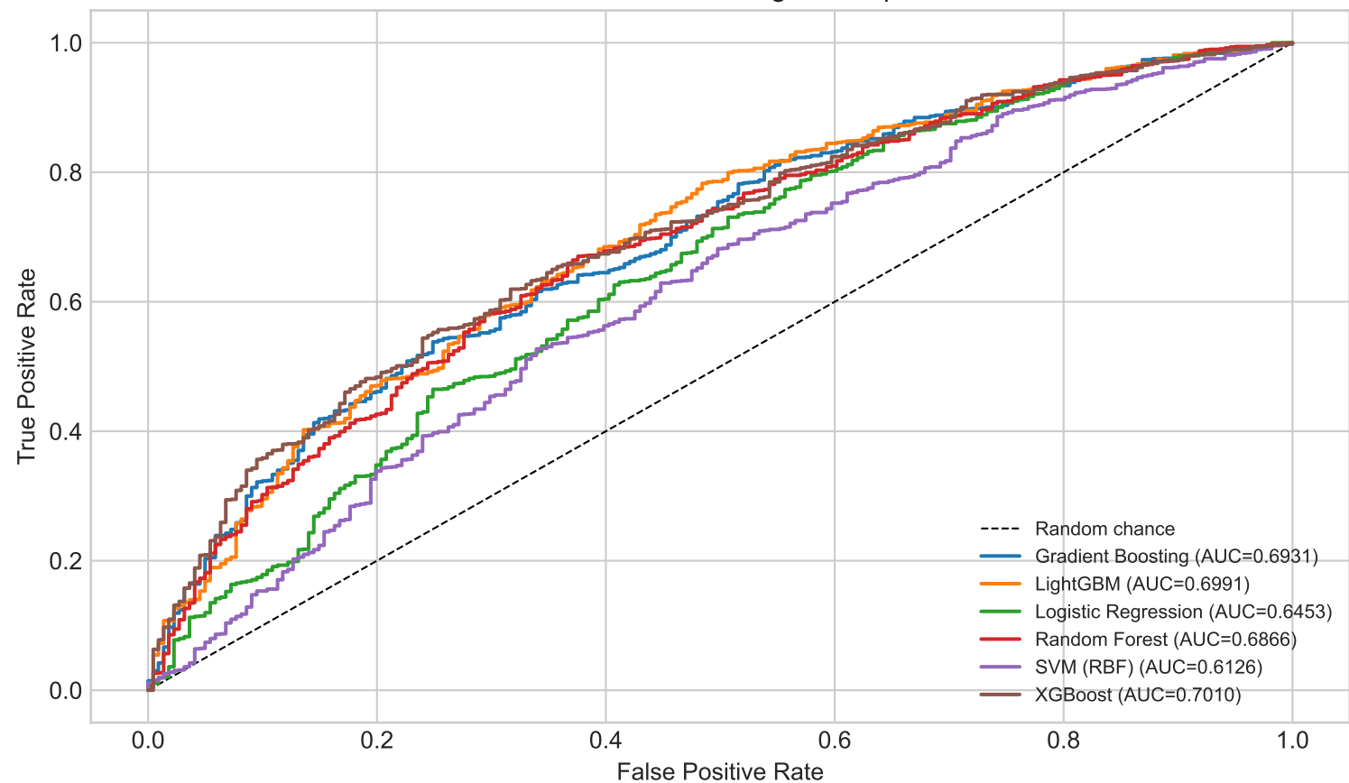
ROC Curves — Best Configuration per Model
