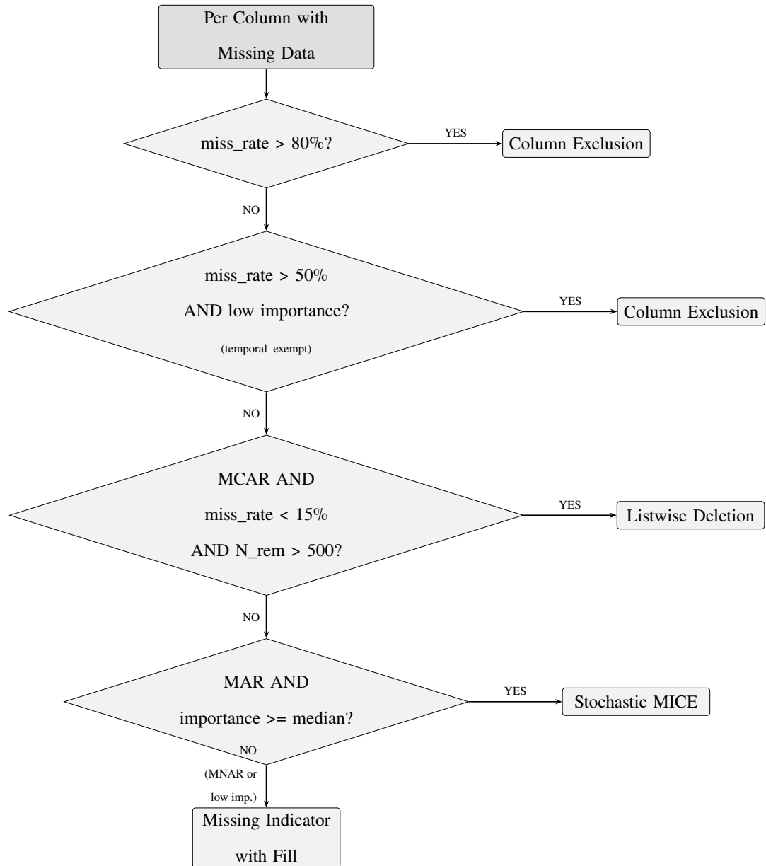
Missing Data Handling Decision Logic
