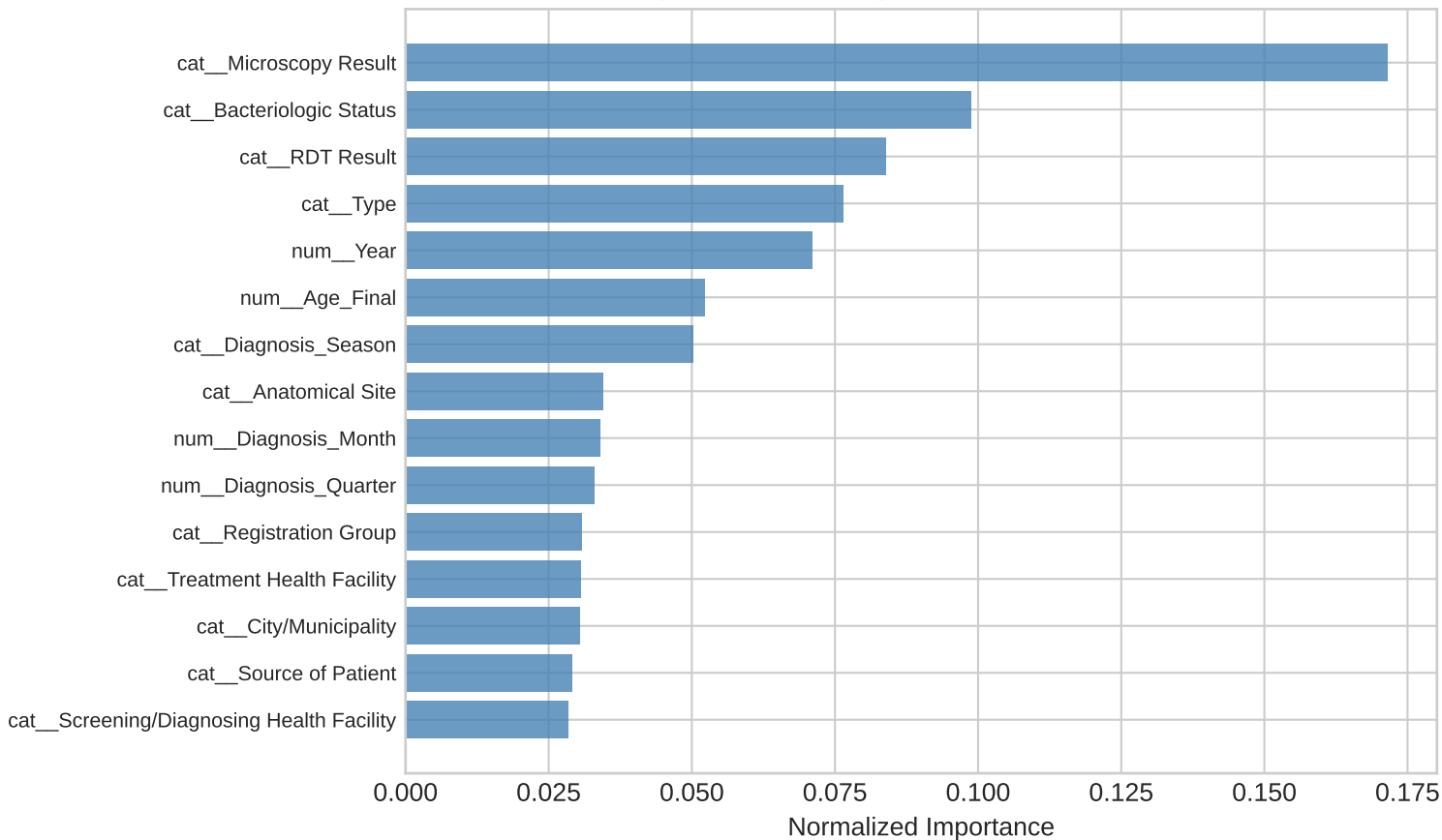
Top 15 Feature Importances — Best Model
