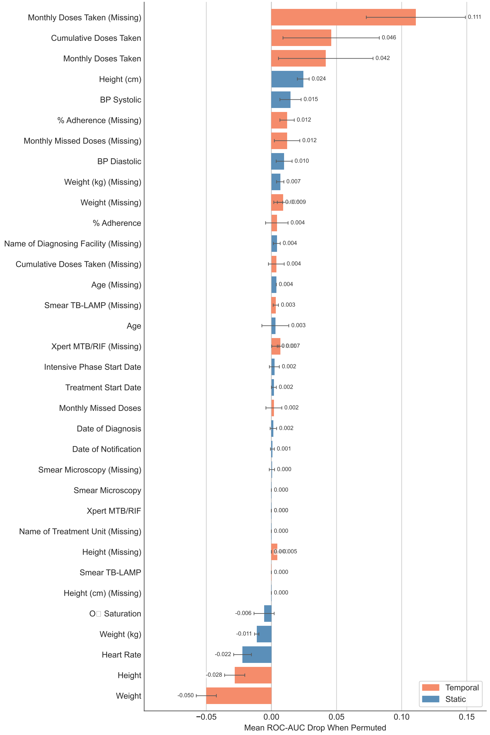
Permutation Feature Importances — Hybrid Bi-LSTM (Best Model)
