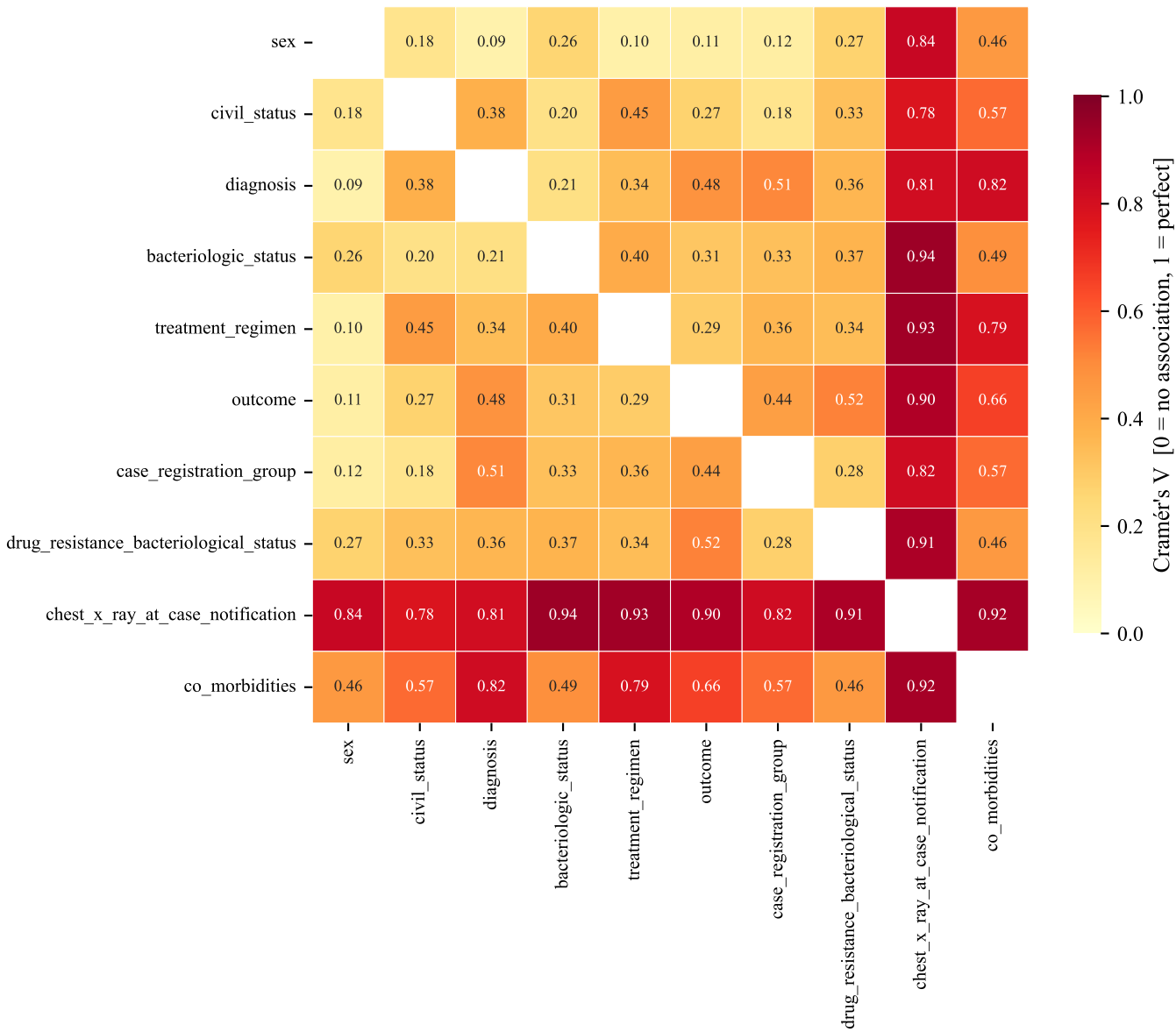
Cramér's V — Raw Categorical Features (white cells = NaN)
