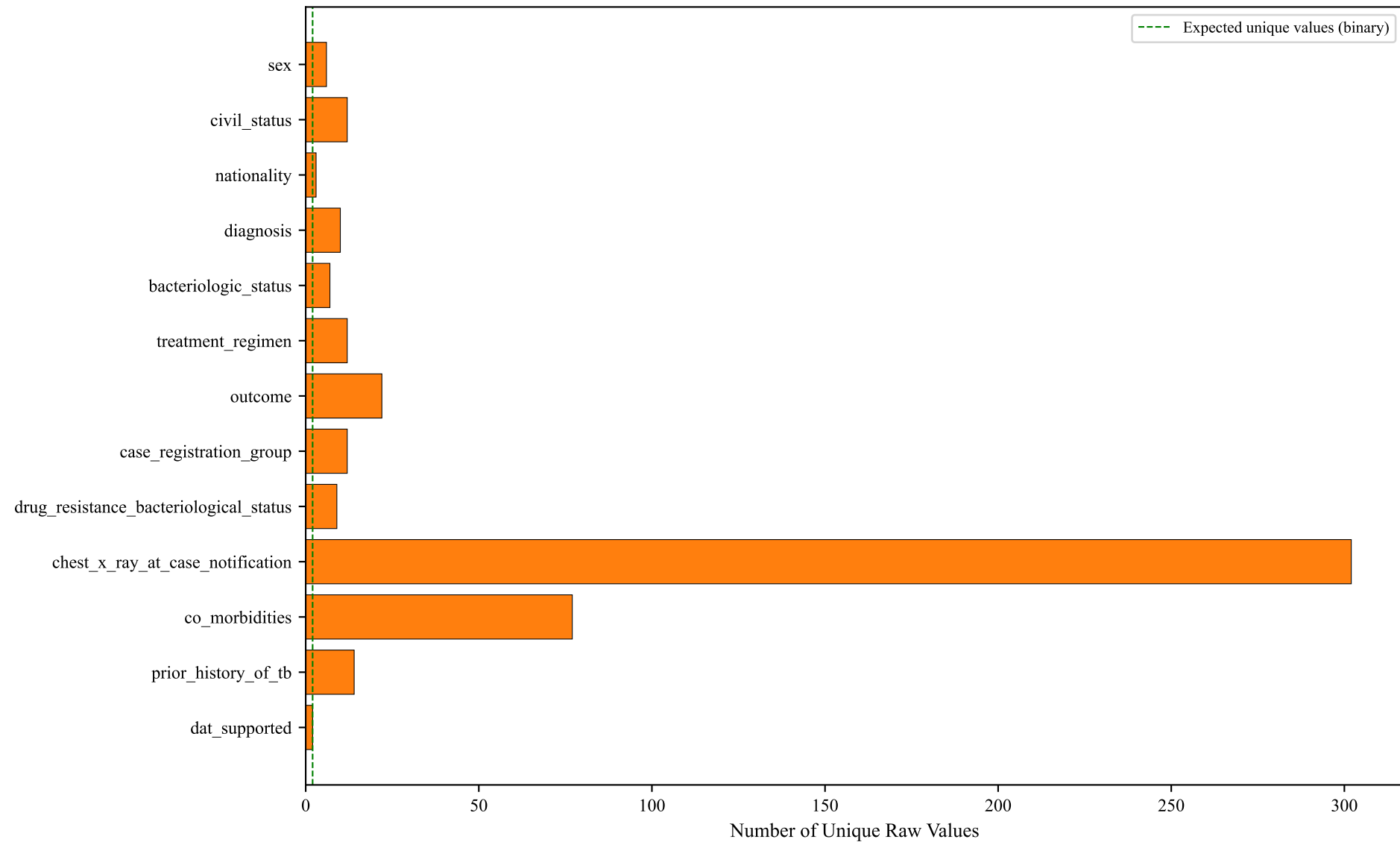
Categorical Feature Raw Cardinality High cardinality indicates inconsistent coding requiring harmonization
