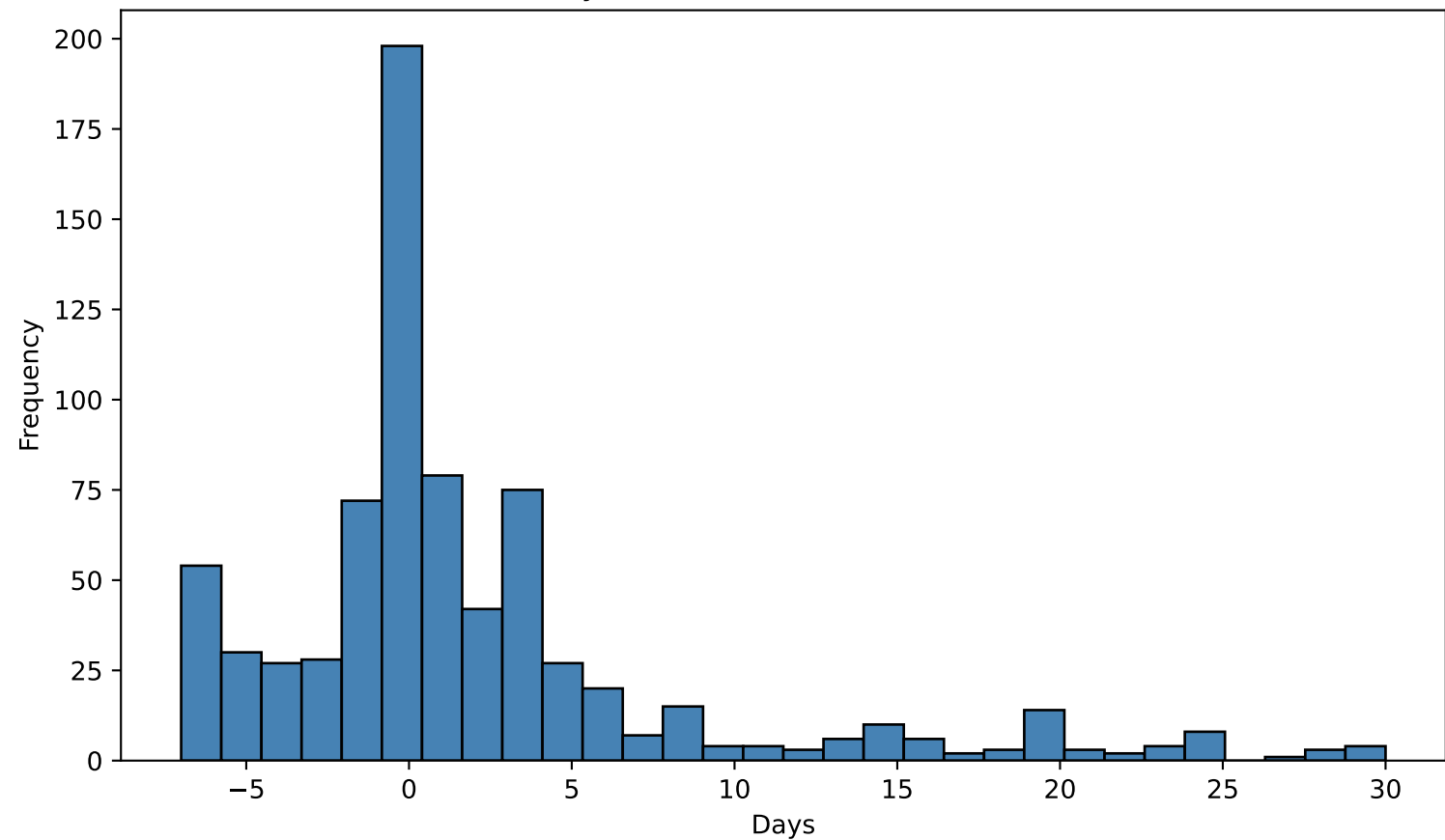
Days To RDT Result Distribution
