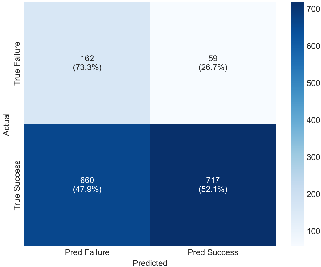
Confusion Matrix — Best Model (Test Set)
