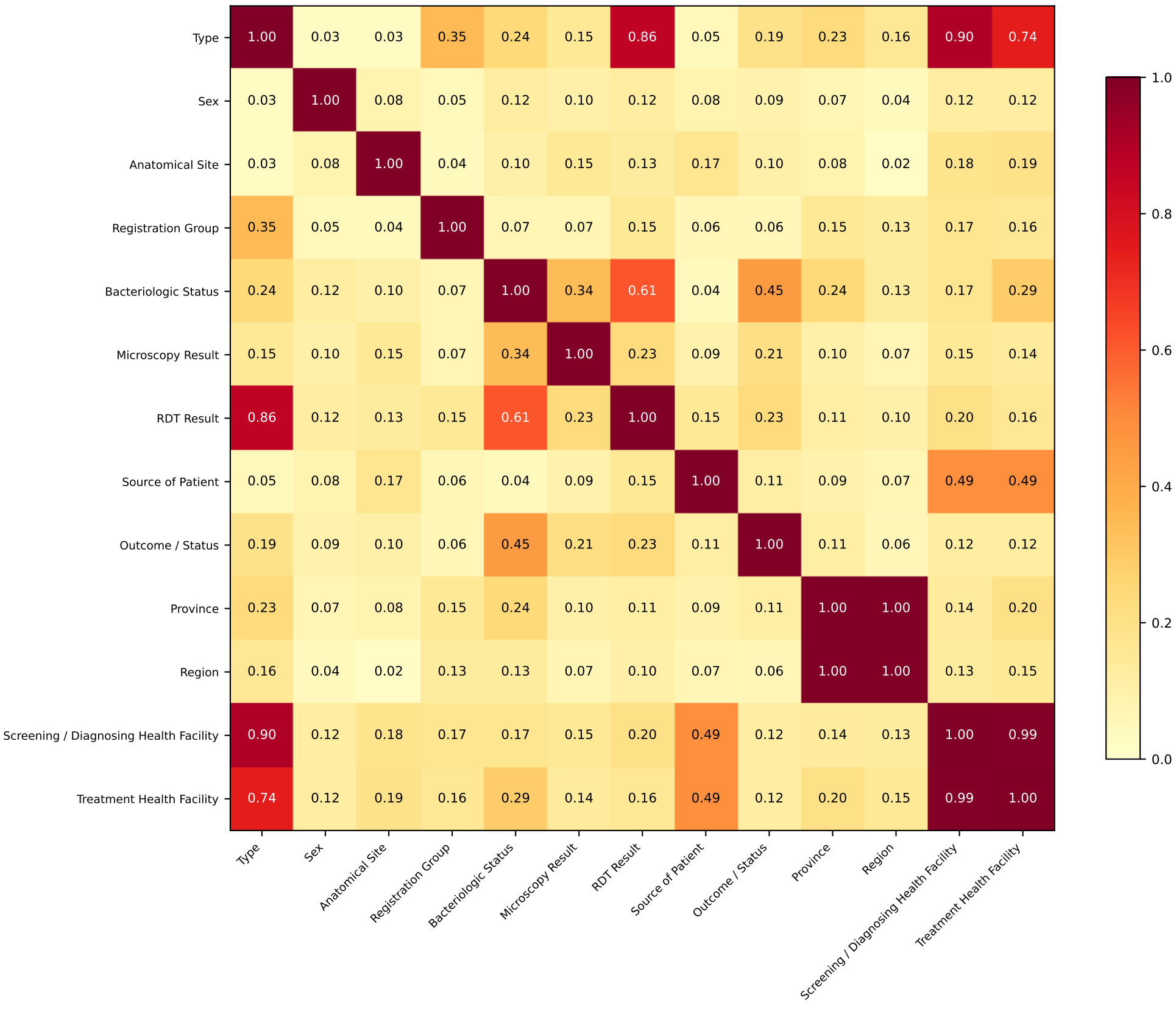
Cramér's V Correlation Matrix of Categorical Variables
