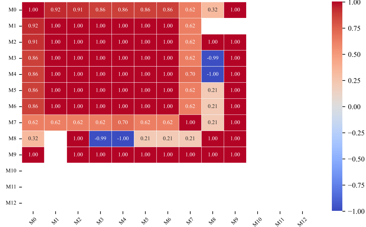
Pairwise Monthly Correlation — Pct Adherence Strong off-diagonal values support temporal modelling
