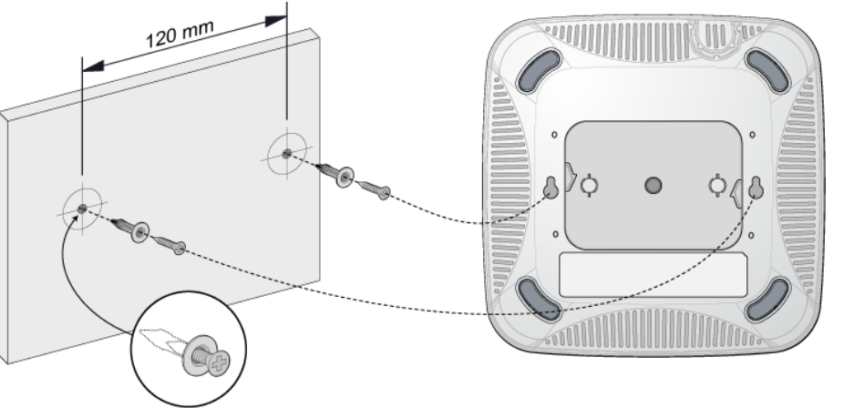
Figure 7 Mounting Using the Integrated Wall-Mounting Slots
