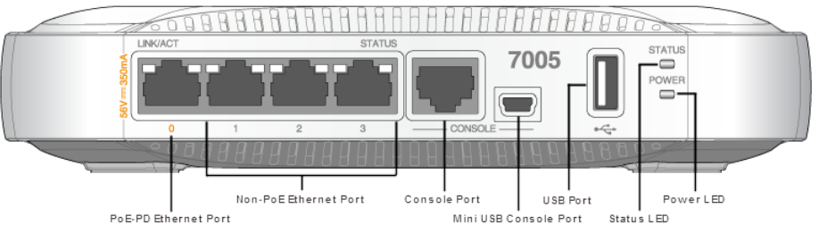
Figure 2 Back Panel of the 7005 Controller
