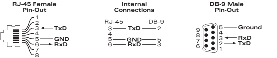
Figure 5 RJ-45 (Female) to DB9 (Male) Modular Adapter Conversion
