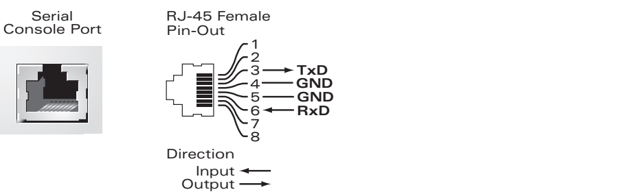
Figure 4 Serial Console Port Pin-Out
