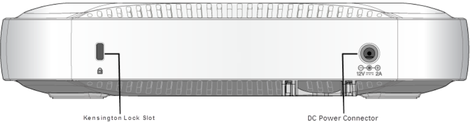
Figure 2 Back Panel of the 7005 Controller
