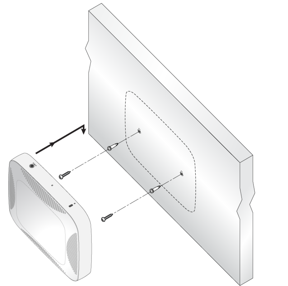
Figure 8 Wall Mounting HPE Aruba Networking 7005
