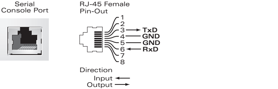
Figure 4 Serial Console Port Pin-Out
