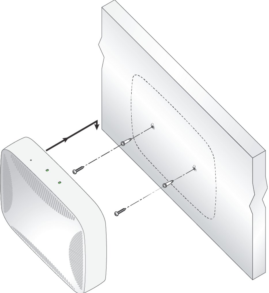
Figure 7 Wall Mounting HPE Aruba Networking 7008
