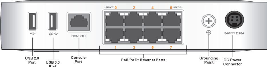
Figure 2 Back Panel of the 7008 Controller
