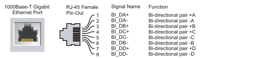
Figure 3 Gigabit Ethernet Port Pin-Out
