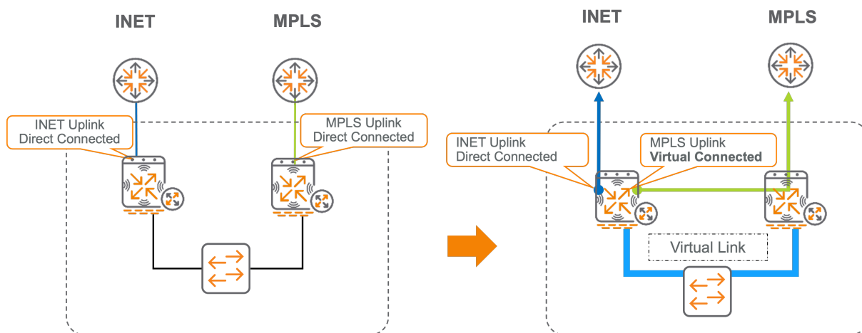
Figure 44: Uplink_Sharing
