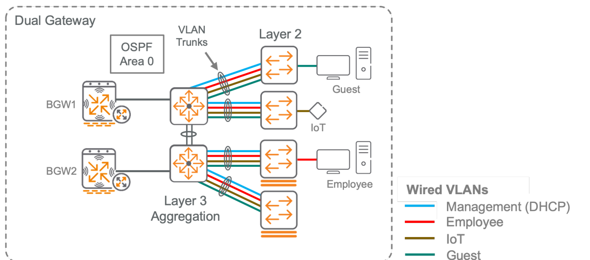
Figure 49: Non-Tunneled L3 Wired Access
