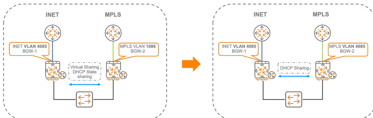
Figure 45: Uplink_Sharing
