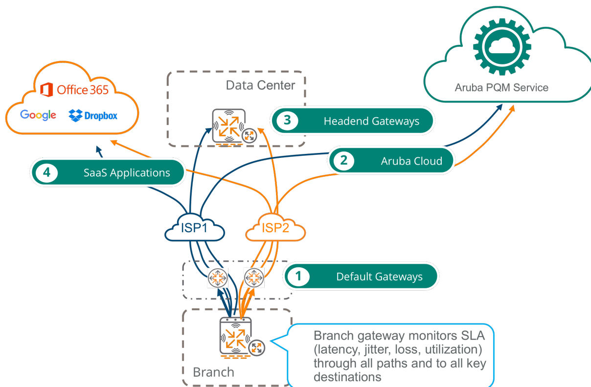
Figure 32: Active Monitoring
