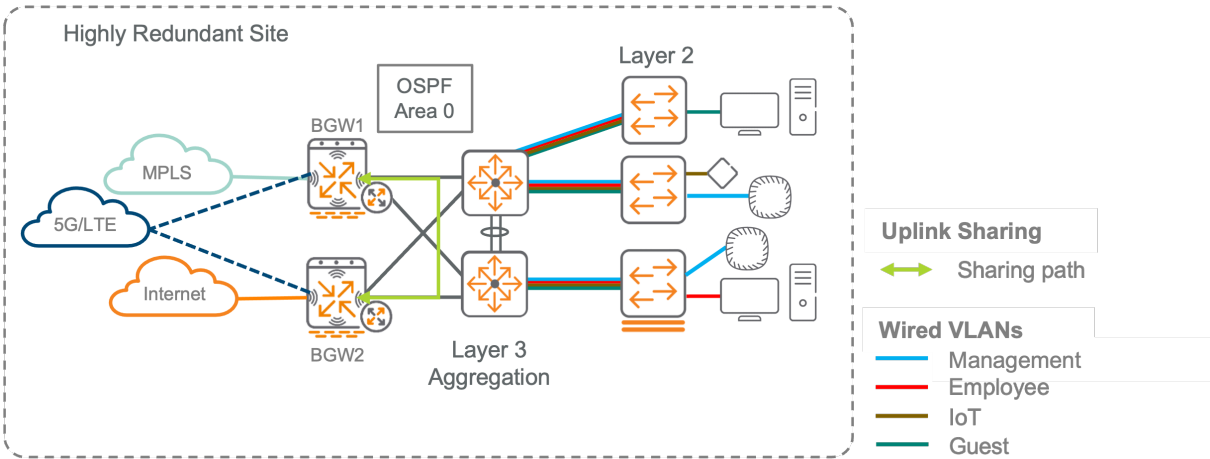
Figure 59: large_site_ra
