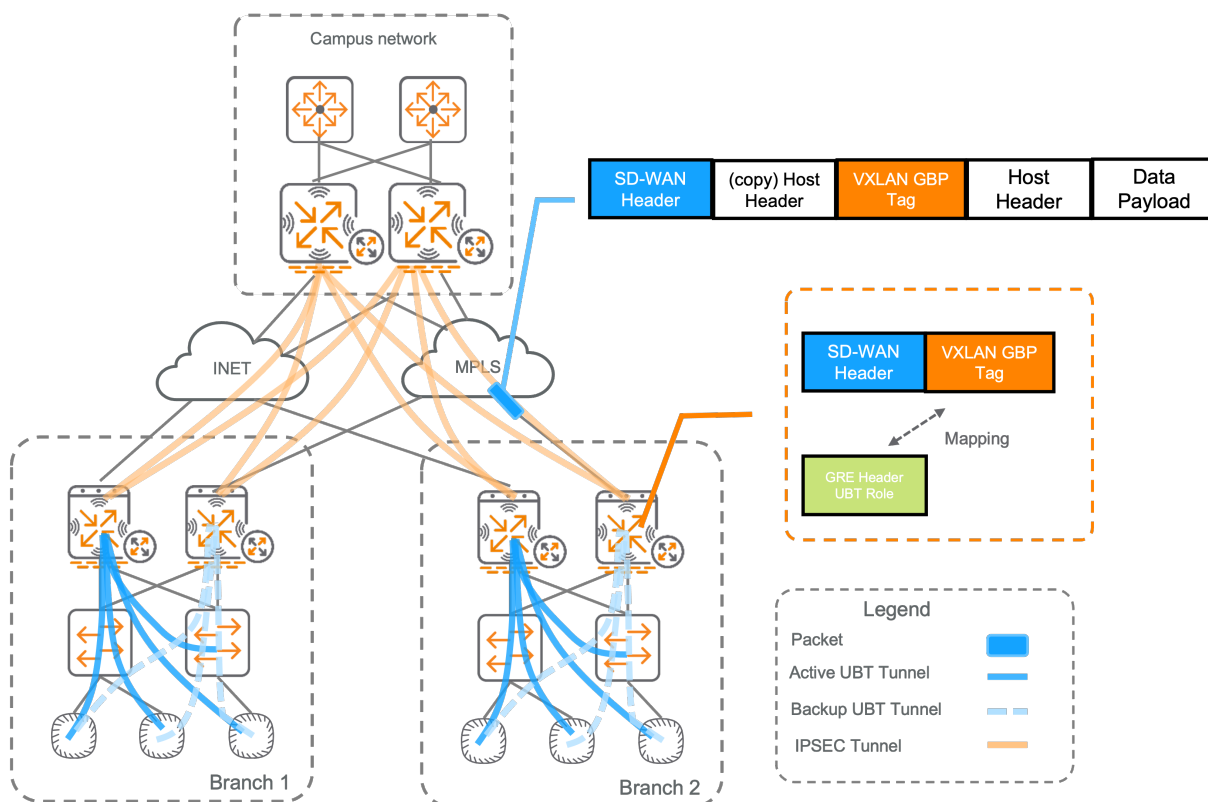
Figure 51: Centralized_Multi_fabric
