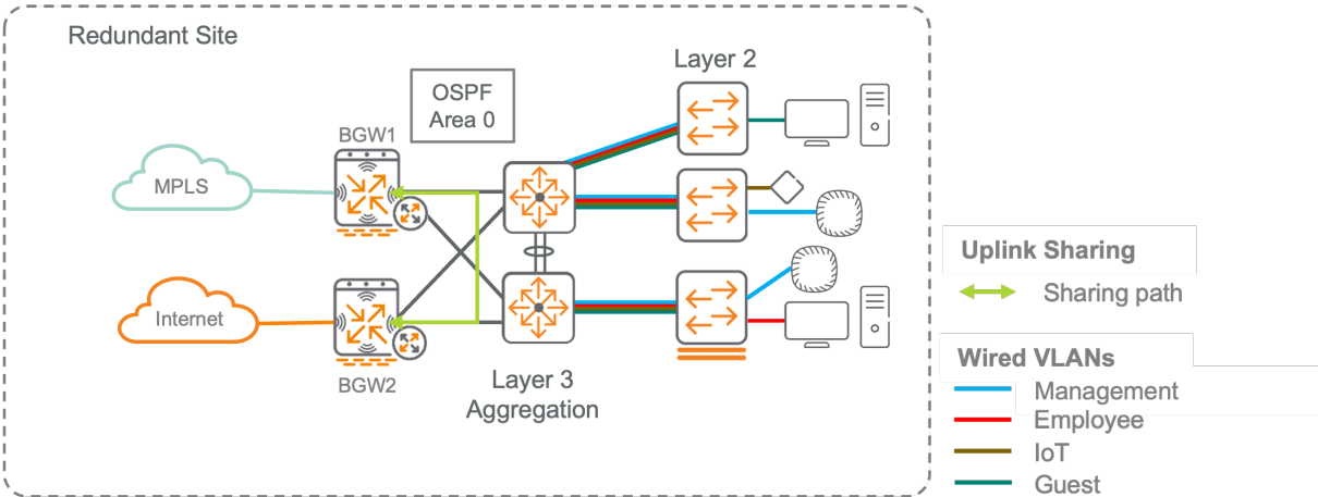
Figure 60: medium_site_ra
