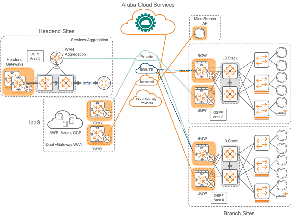
Figure 27: gateway_placement
