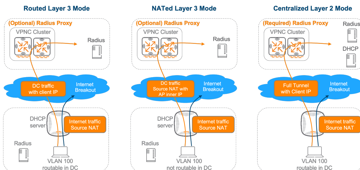
Figure 52: Microbranch_comparison
