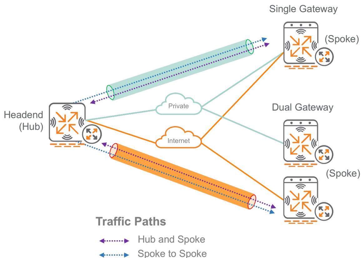
Figure 28: Hub-and-Spoke
