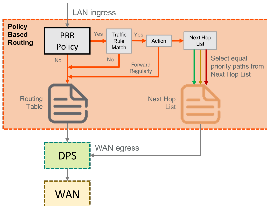
Figure 34: PBR on LAN Ingress
