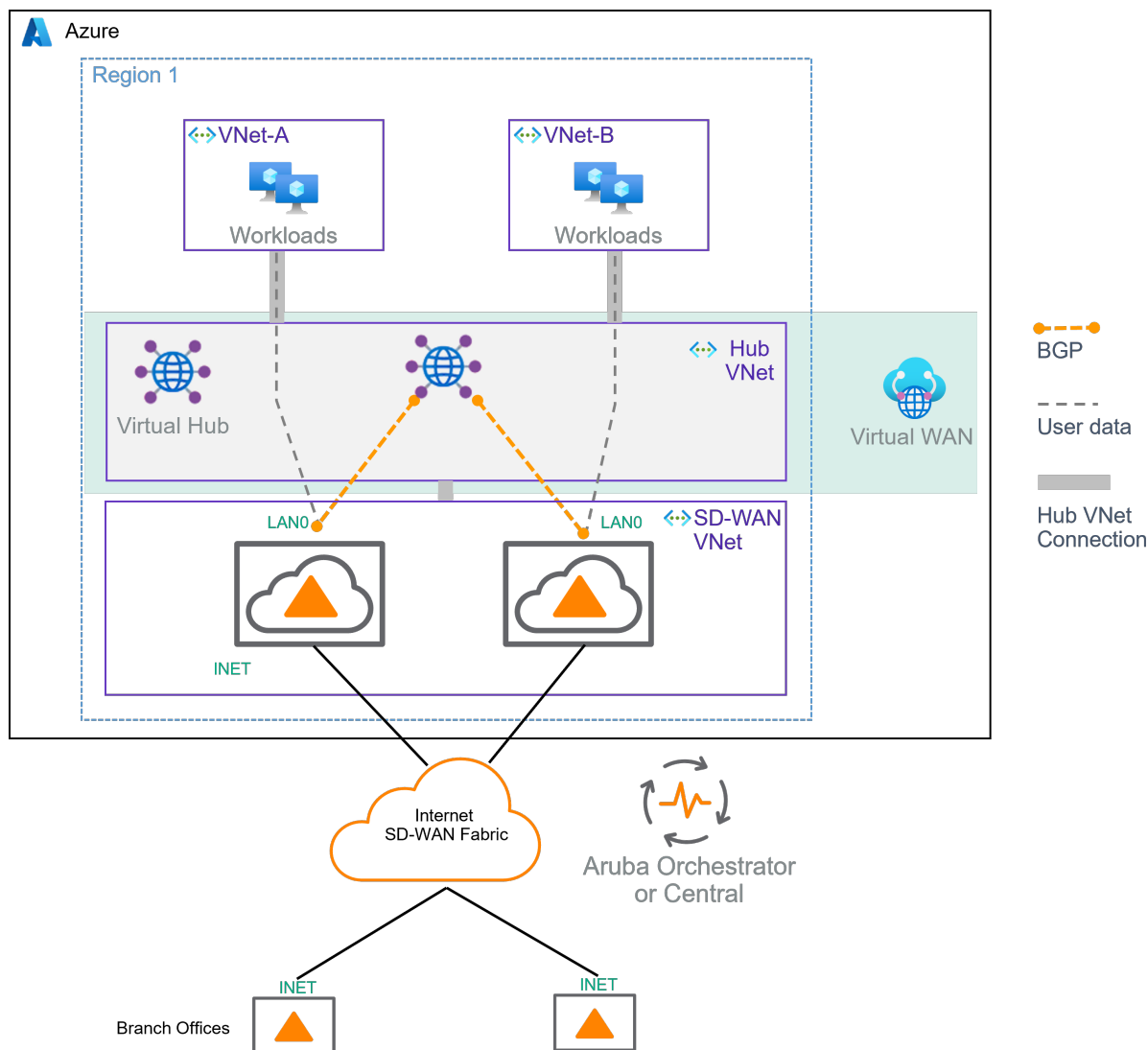
Figure 4: Cloud Integrations
