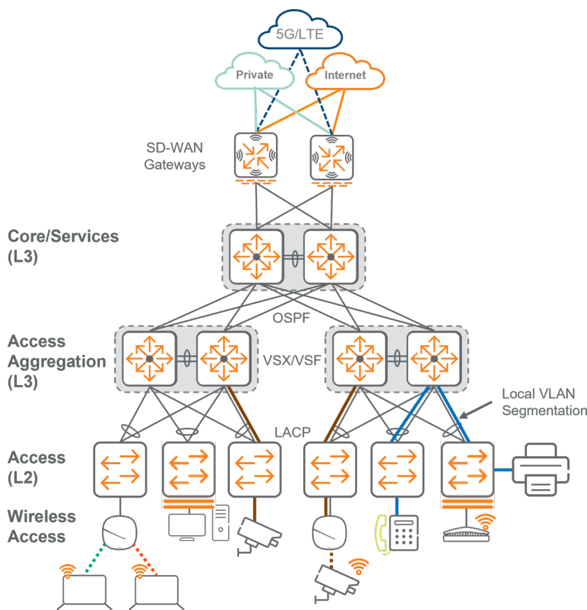
Figure 1: Inline Deployment
