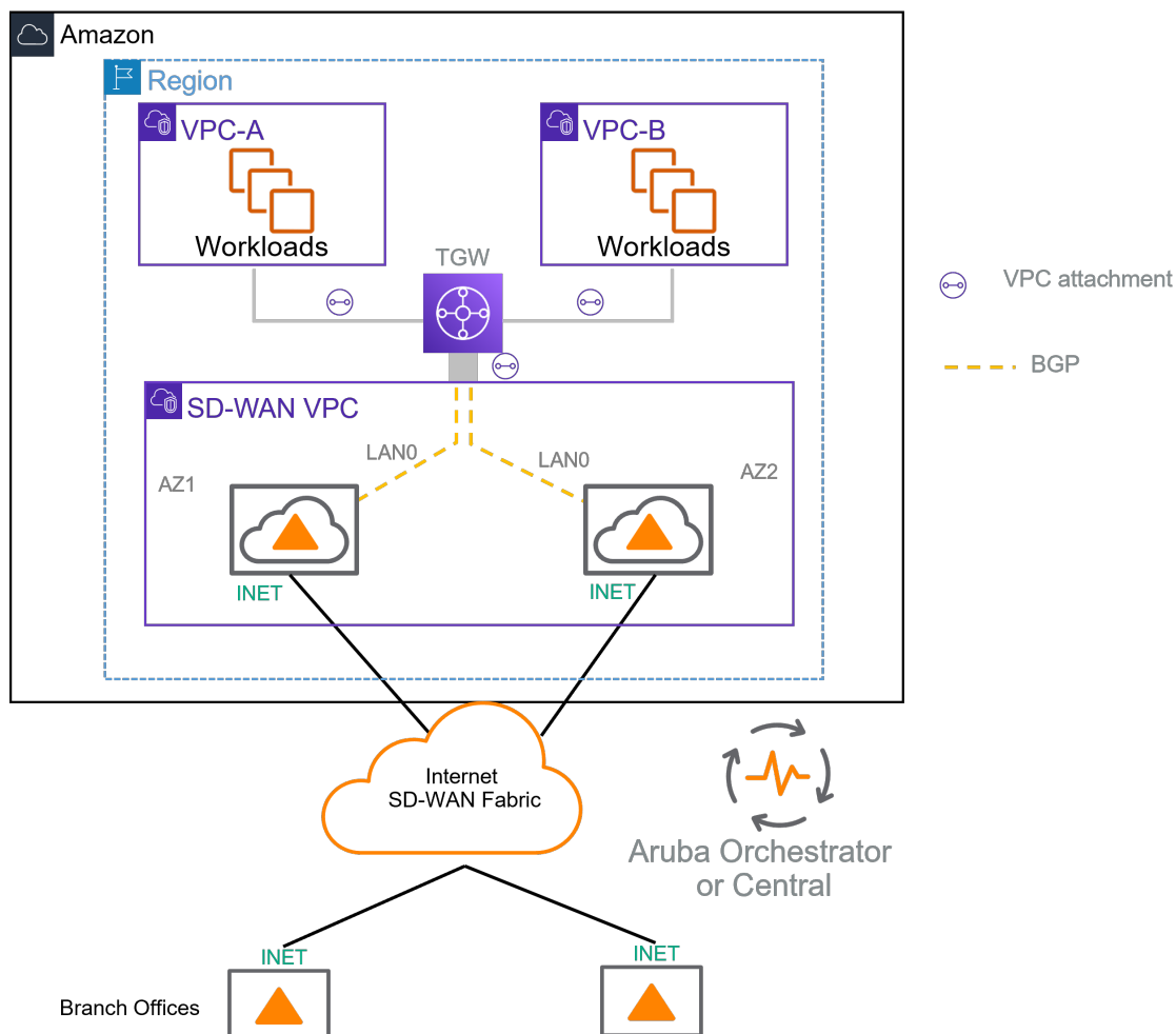
Figure 5: Cloud Integrations
