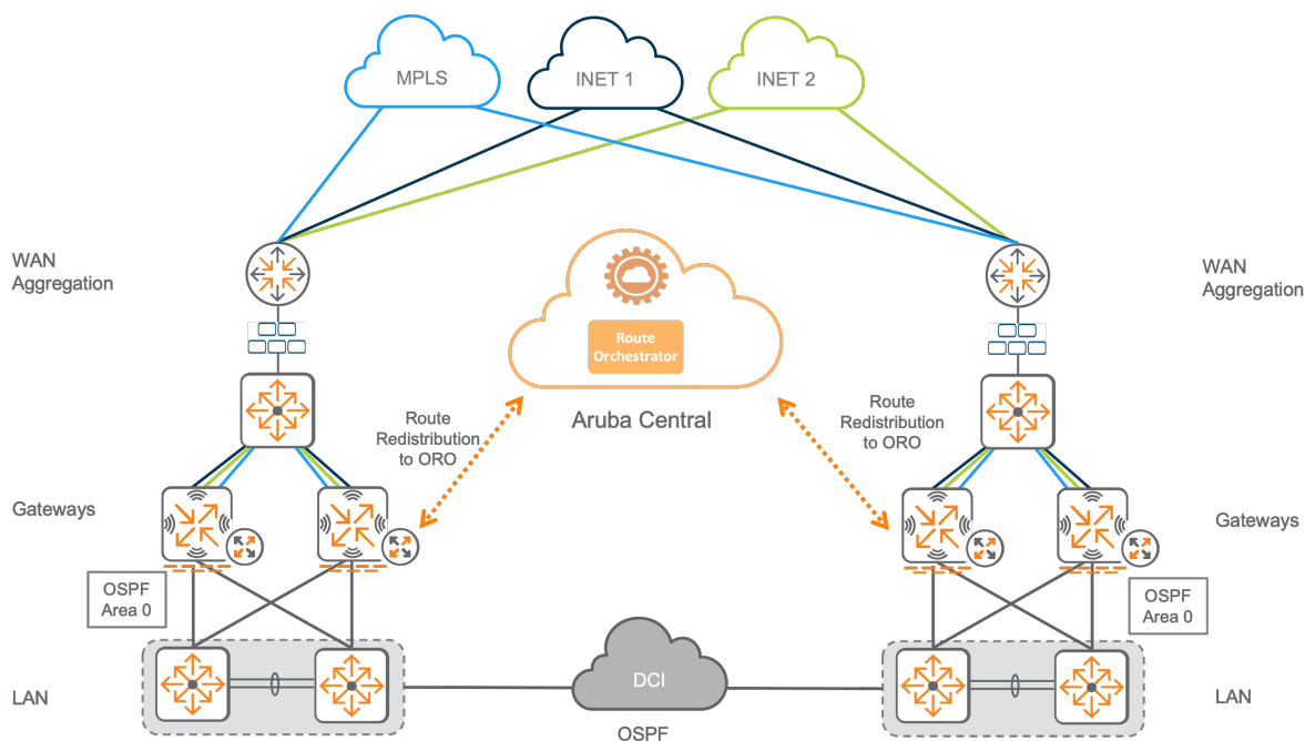
Figure 58: hub_desgin_ra
