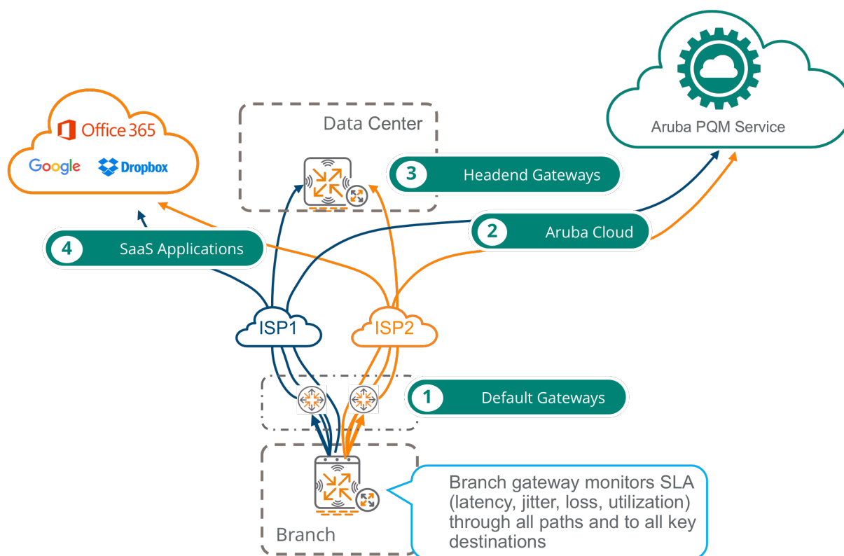
Figure 32: Active Monitoring
