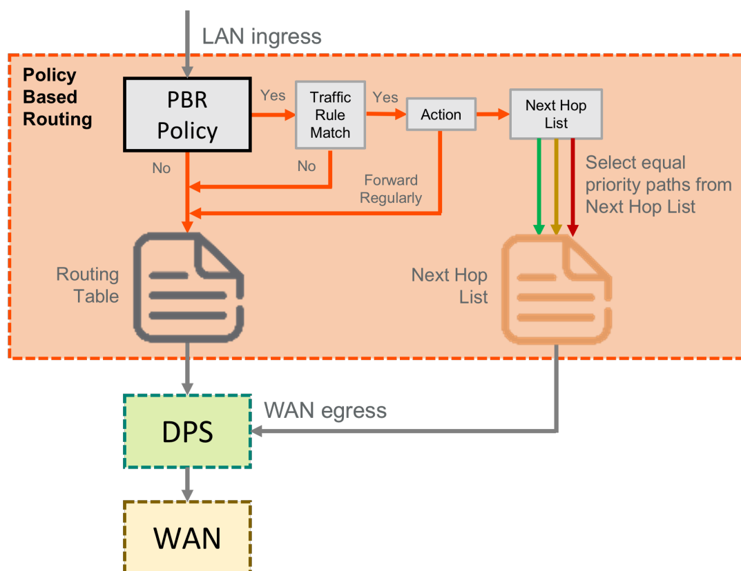
Figure 34: PBR on LAN Ingress
