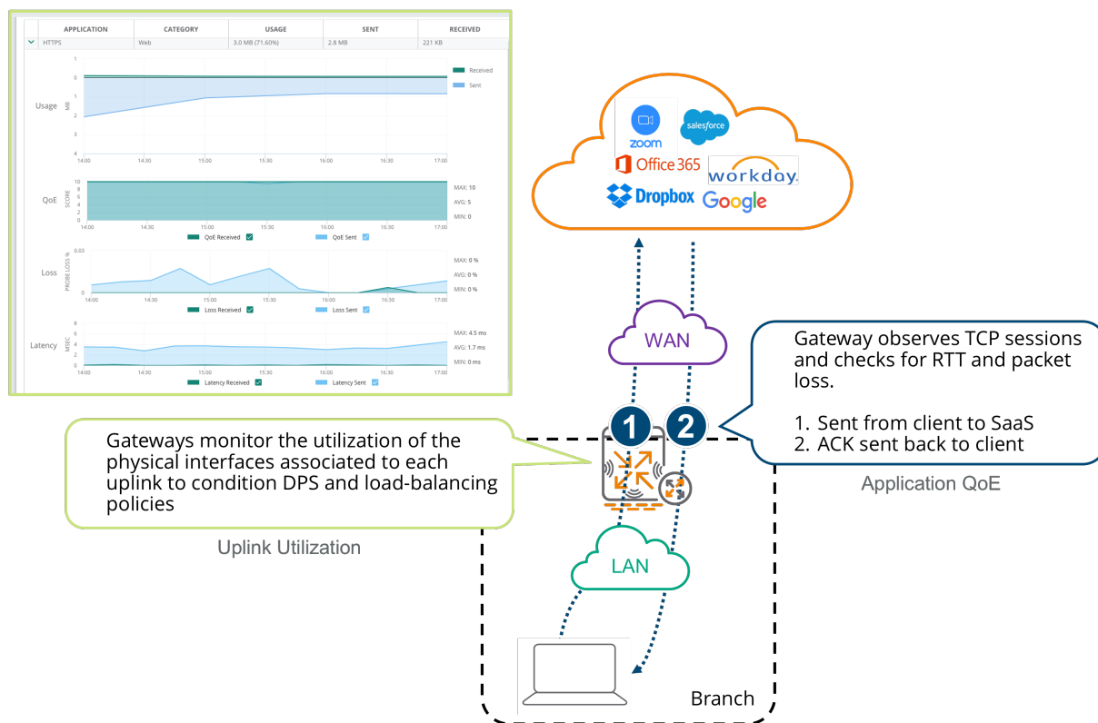
Figure 33: Passive Monitoring
