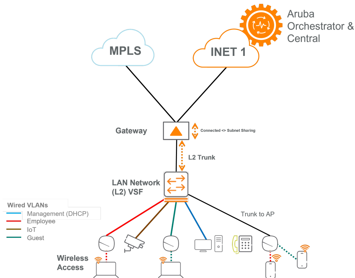
Figure 19: Small Branch Overview
