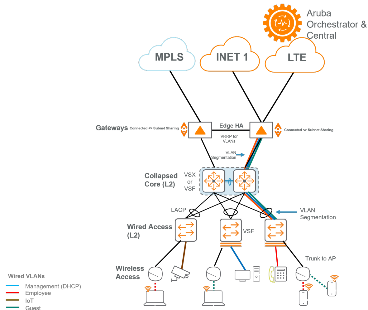
Figure 18: Large Branch Overview
