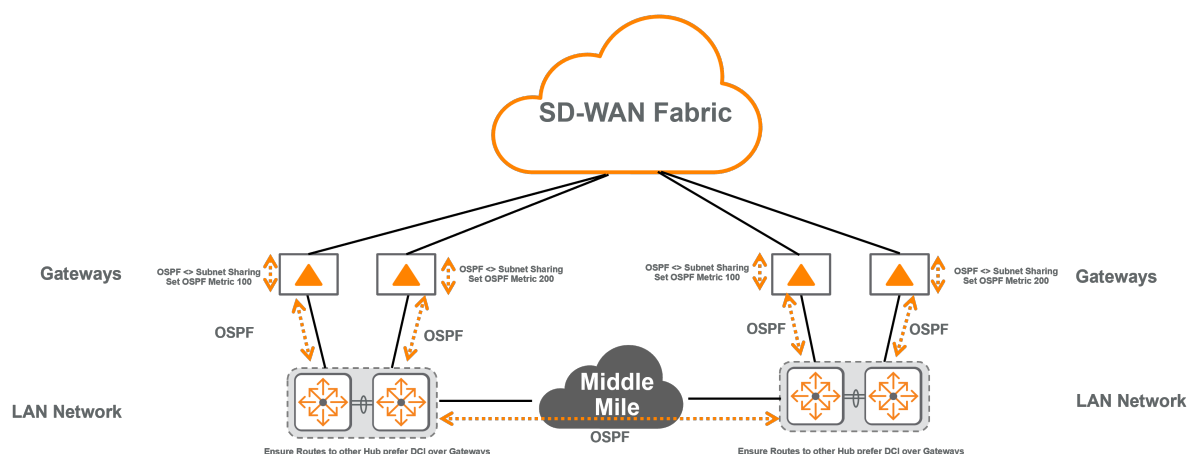
Figure 14: LAN Routing Integration
