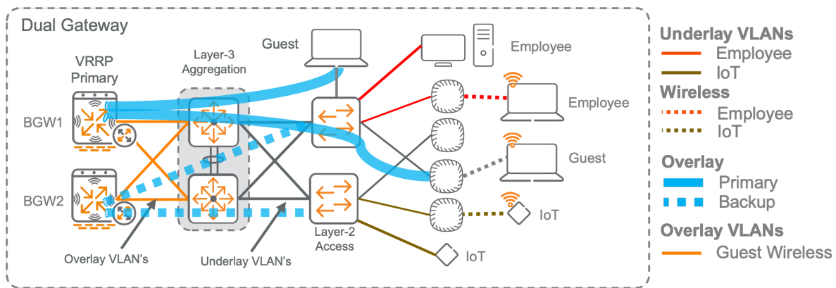
Figure 50: Tunneled Access with Dynamic Segmentation
