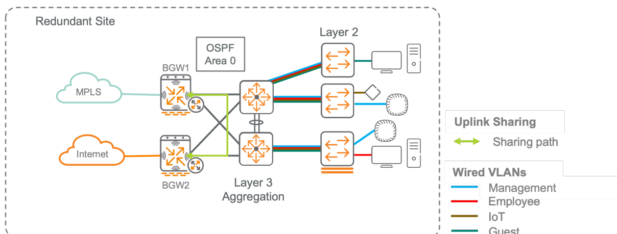
Figure 60: medium_site_ra
