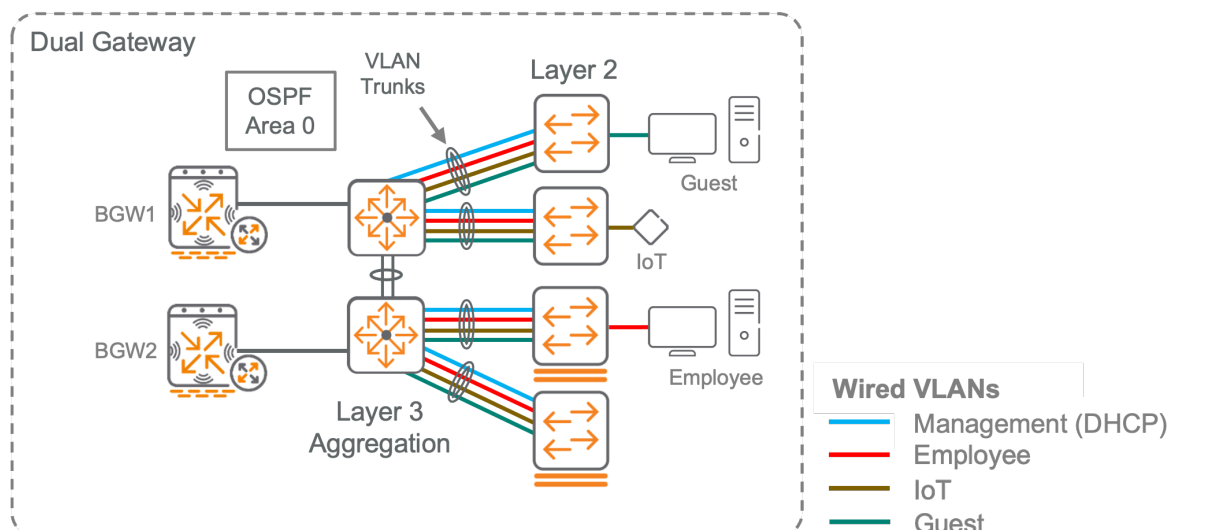
Figure 49: Non-Tunneled L3 Wired Access
