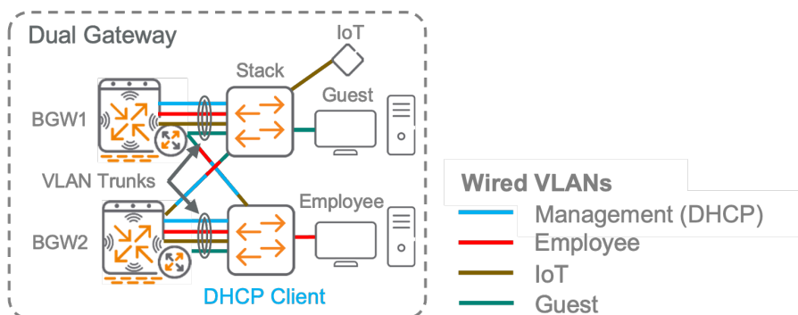
Figure 46: Non-Tunneled L2 Wired Access
