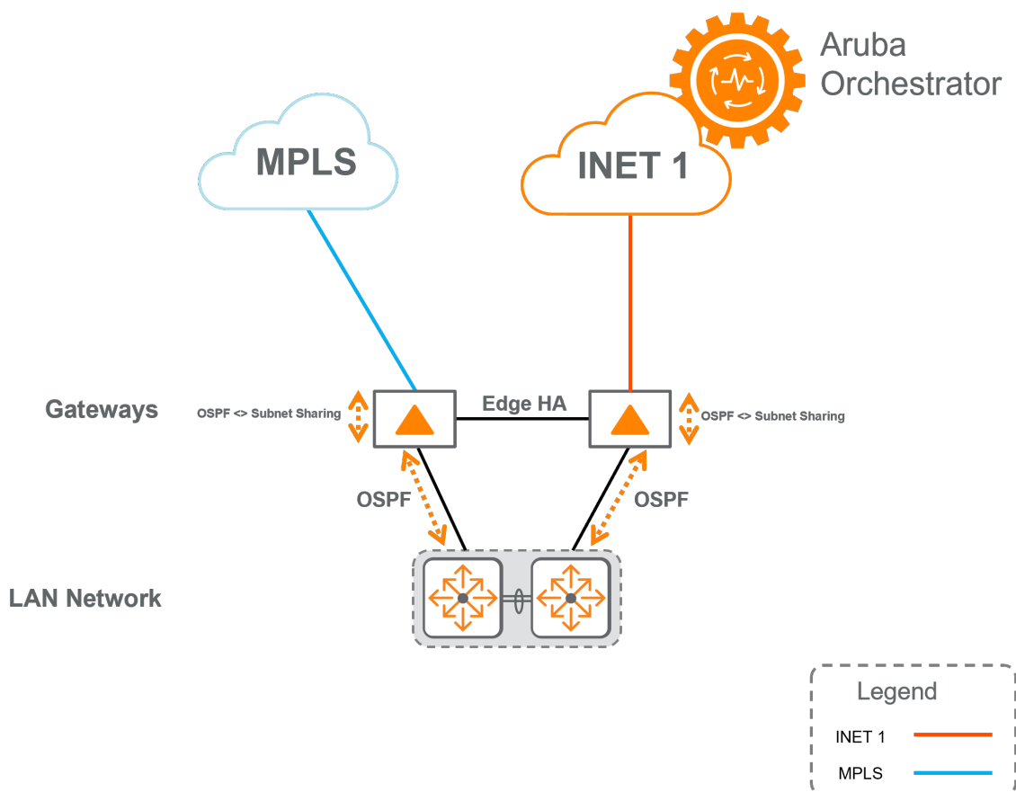
Figure 56: RA - Medium Branch
