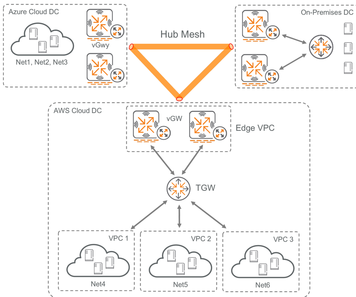
Figure 29: Hub Mesh
