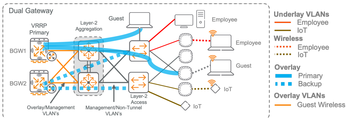
Figure 47: L2_tunneled_ubt
