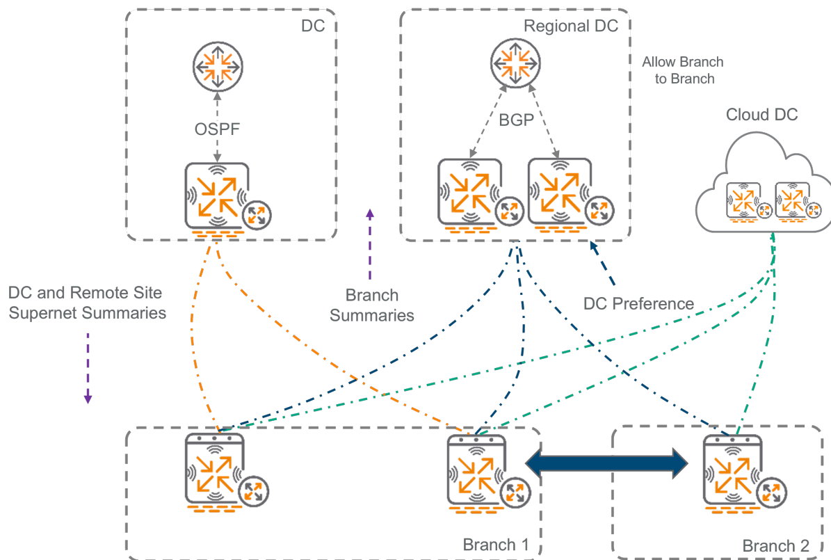
Figure 42: Multiple Active DCs
