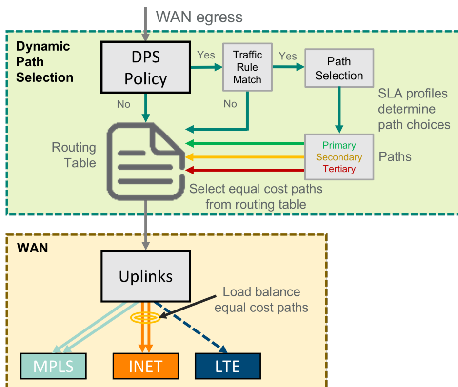
Figure 36: DPS on WAN Egress
