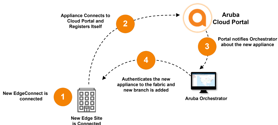
Figure 22: EC ZTP
