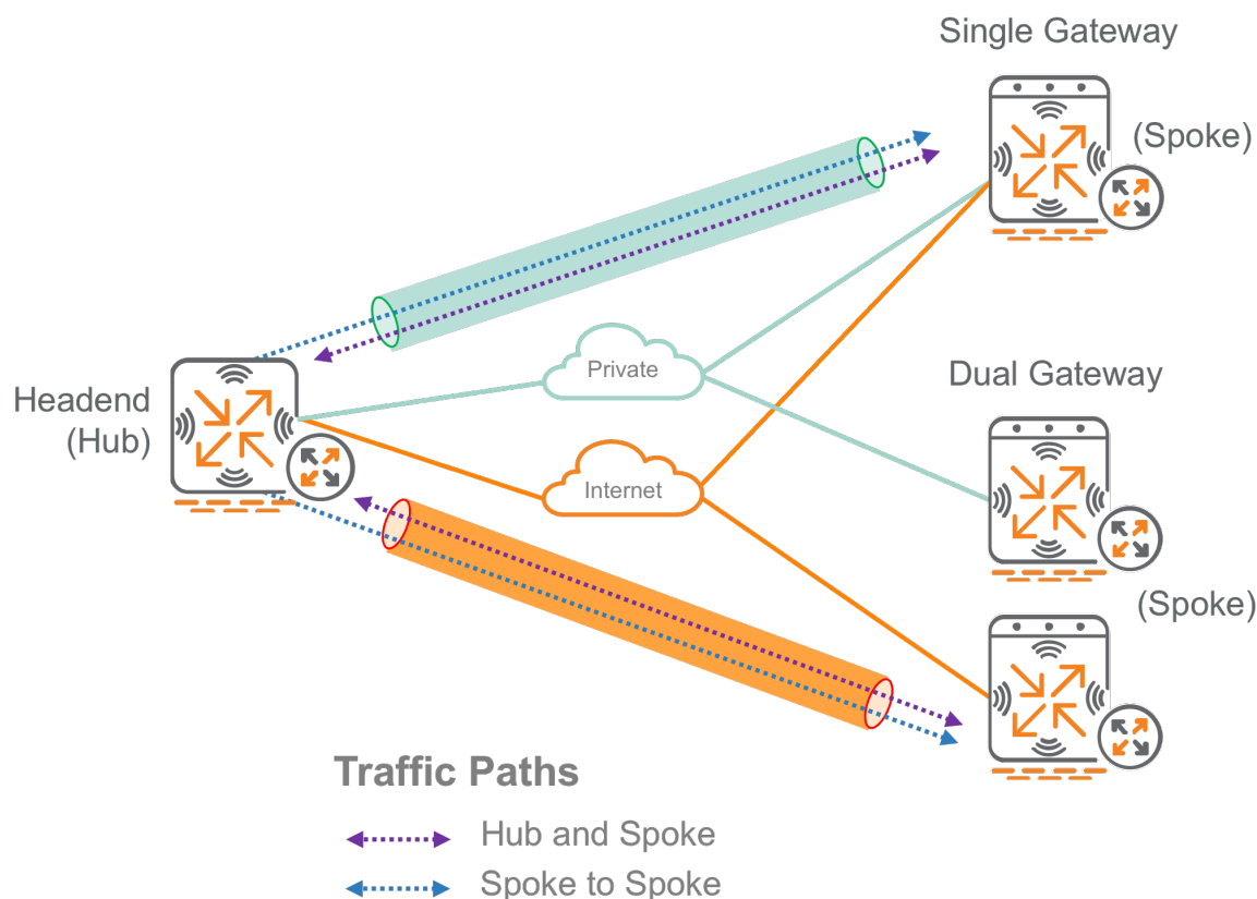
Figure 28: Hub-and-Spoke
