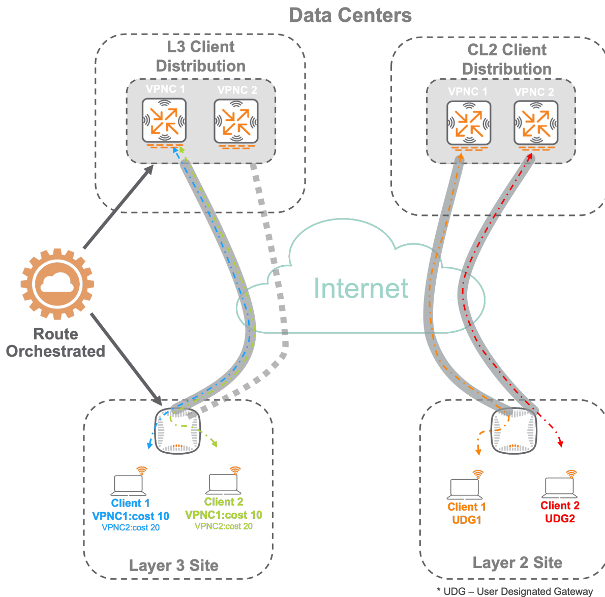
Figure 53: clustering and load balancing
