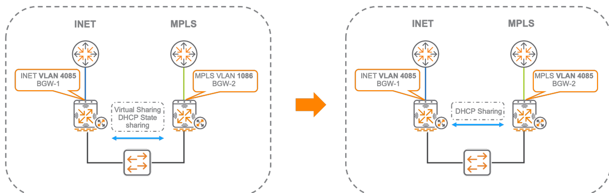
Figure 45: Uplink_Sharing
