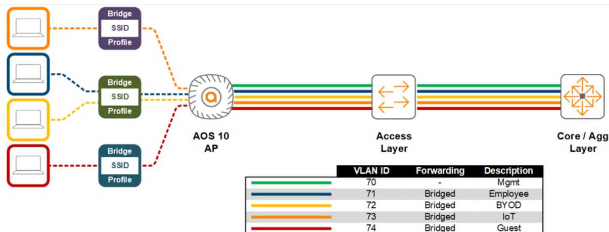
Figure 21: Bridge Mode Wireless
