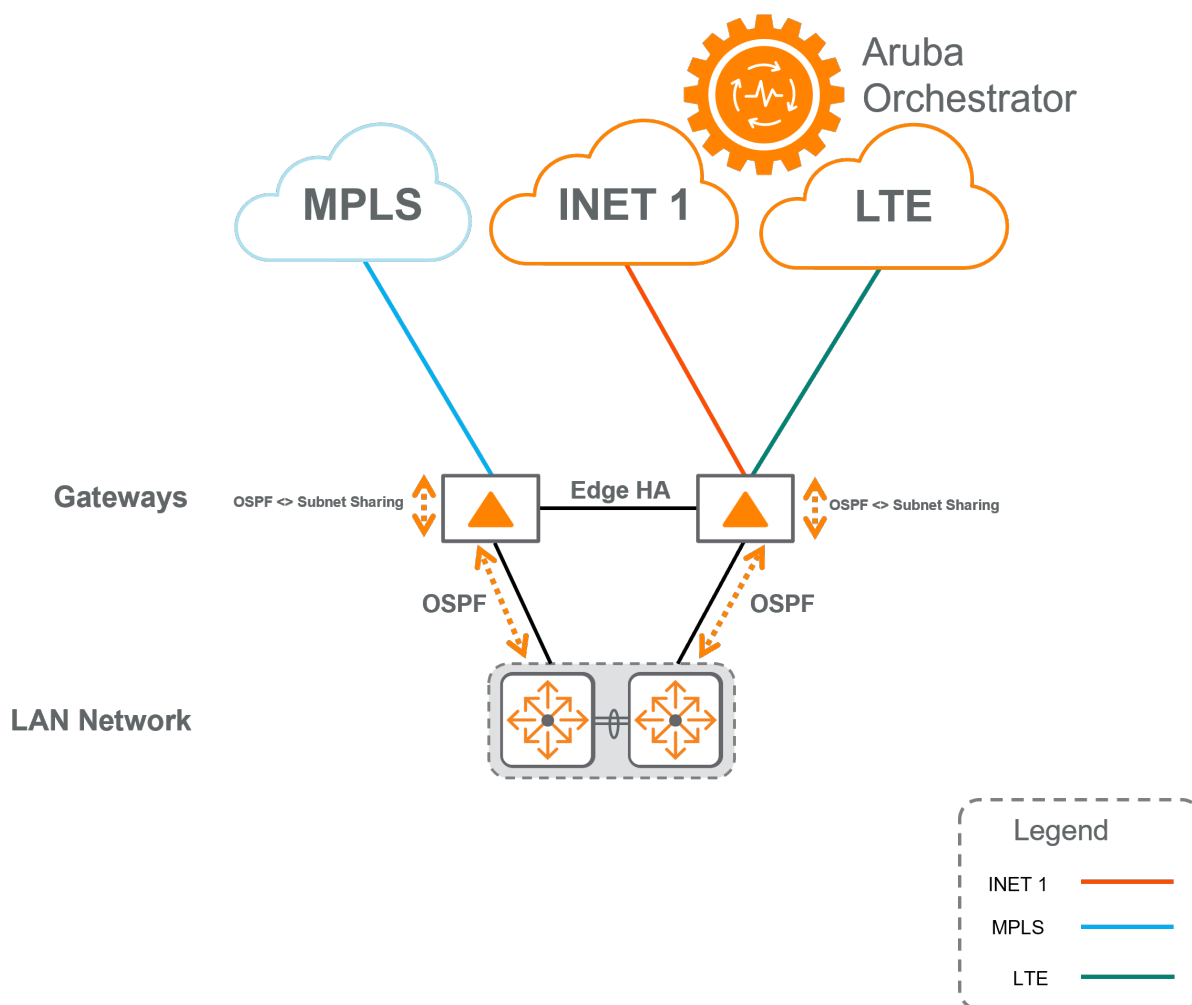
Figure 57: RA - Large Branch
