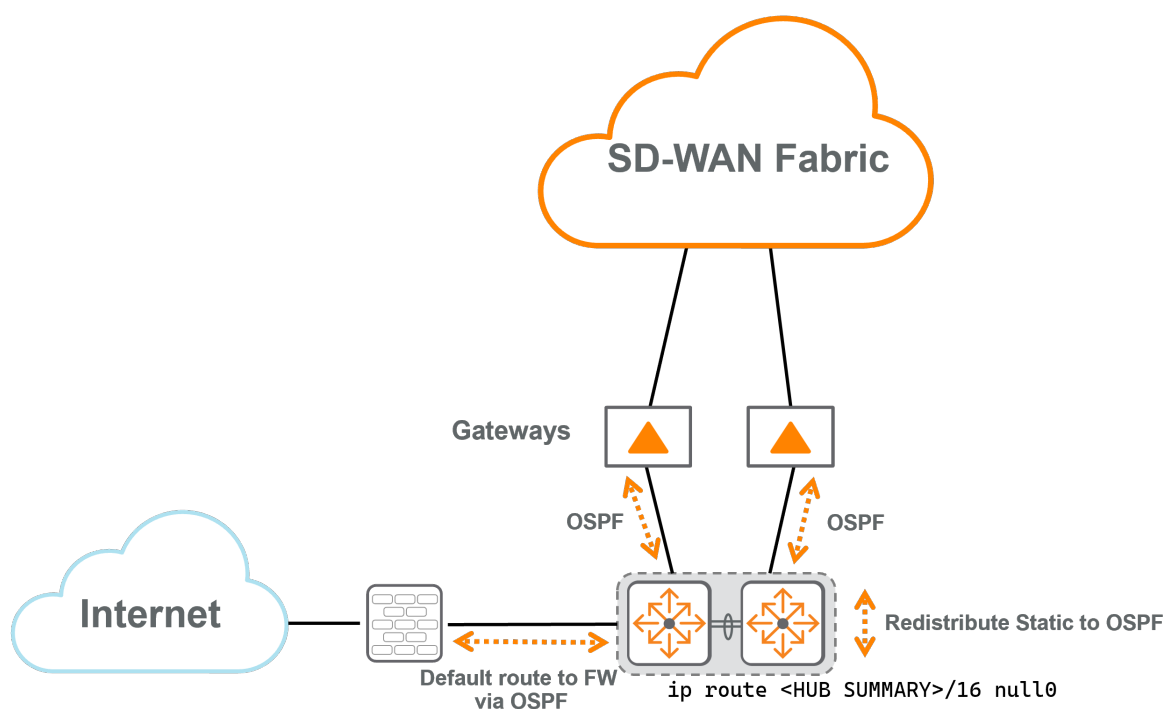
Figure 16: RA - Route Generation
