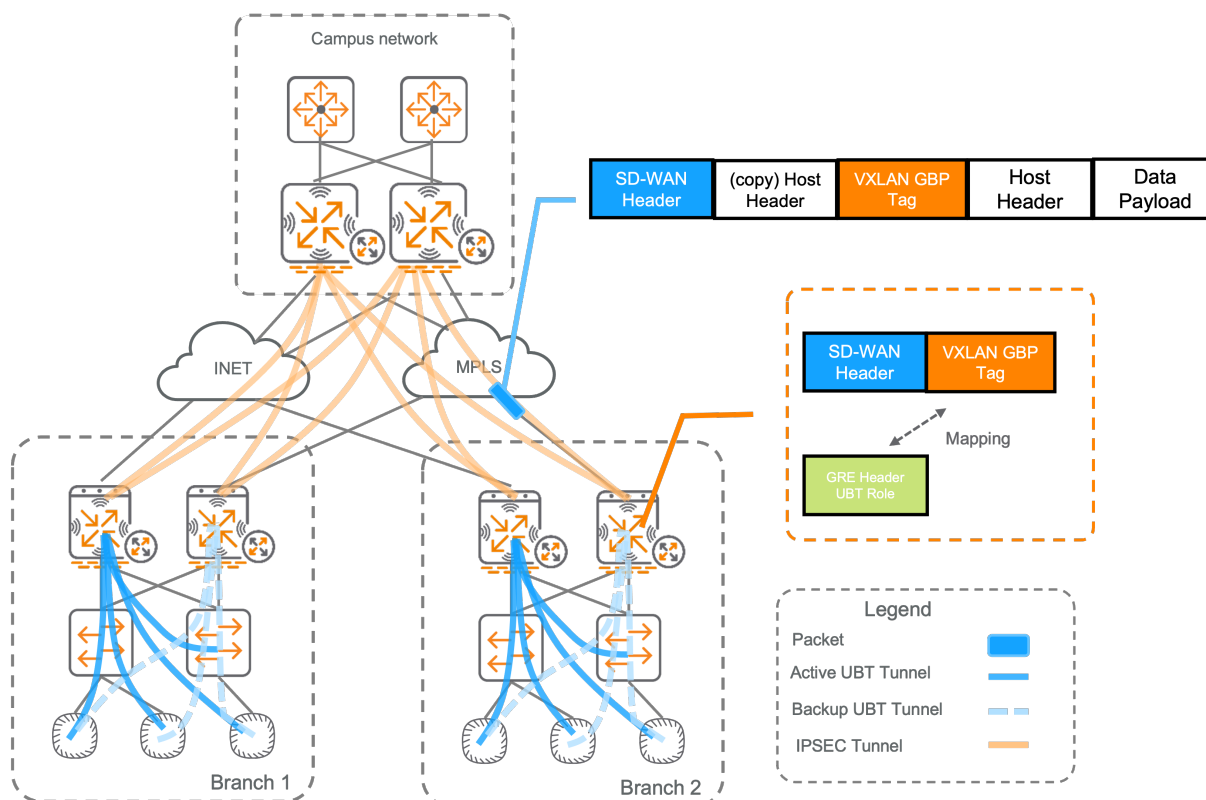
Figure 51: Centralized_Multi_fabric
