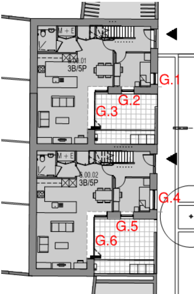
Figure 3 Building 303 Block G – Ground floor plan
