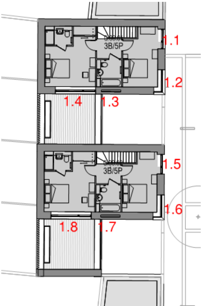
Figure 7 Building 303 Block G – Level 1 floor plan
