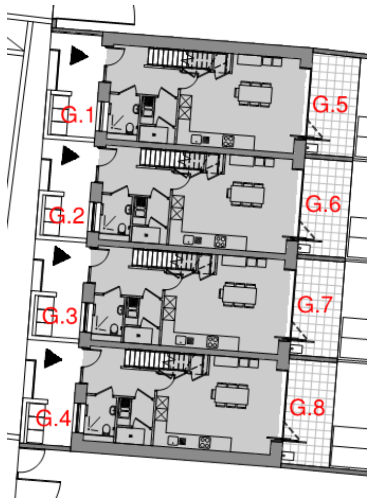
Figure 2 Building 303 Block F– Ground floor plan
