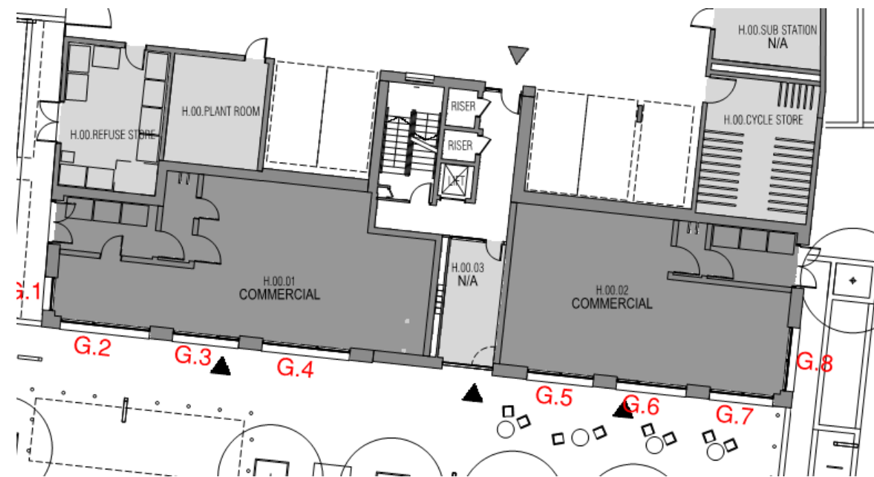
Figure 4 Building 303 Block H – Ground floor plan
