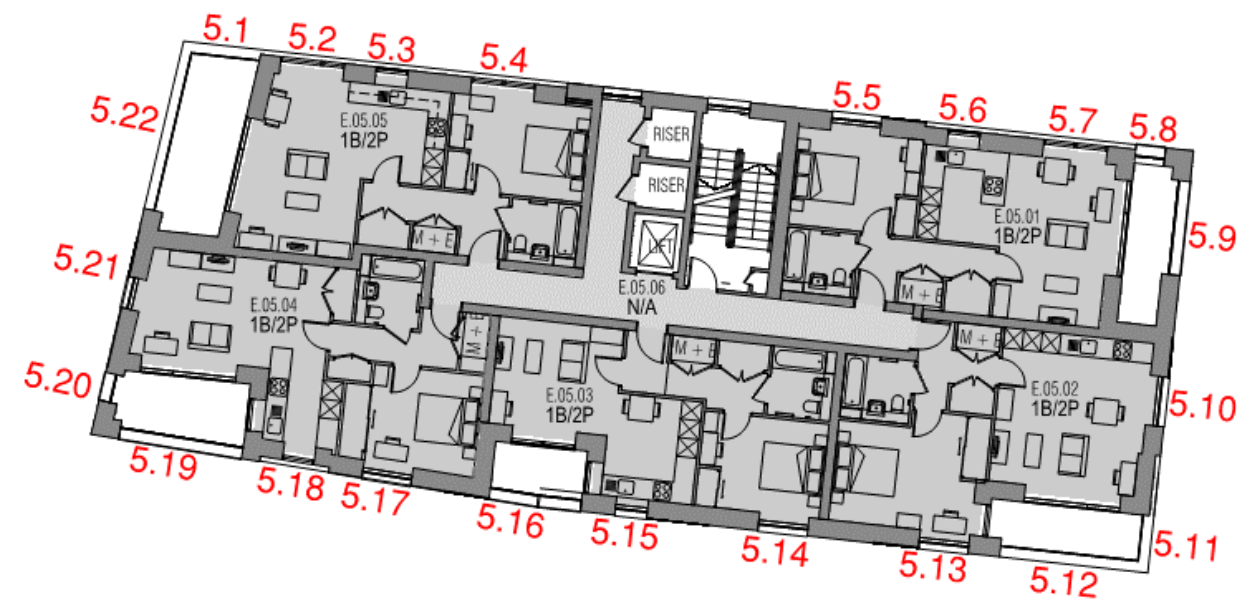
18 Building 303 Block E – Level 5
