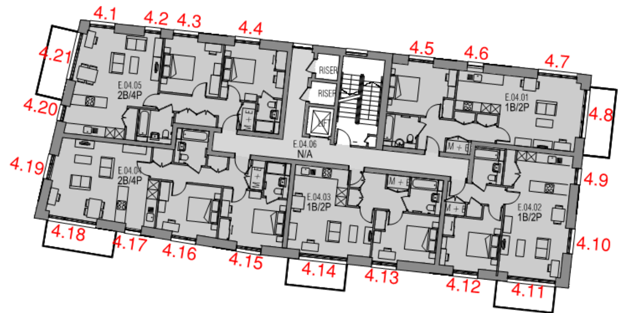
Figure 15 Building 303 Block E– Level 4 floor plan
