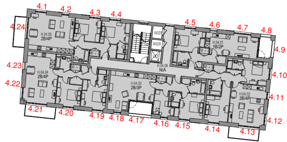
Figure 16 Building 303 Block H– Level 4 floor plan
