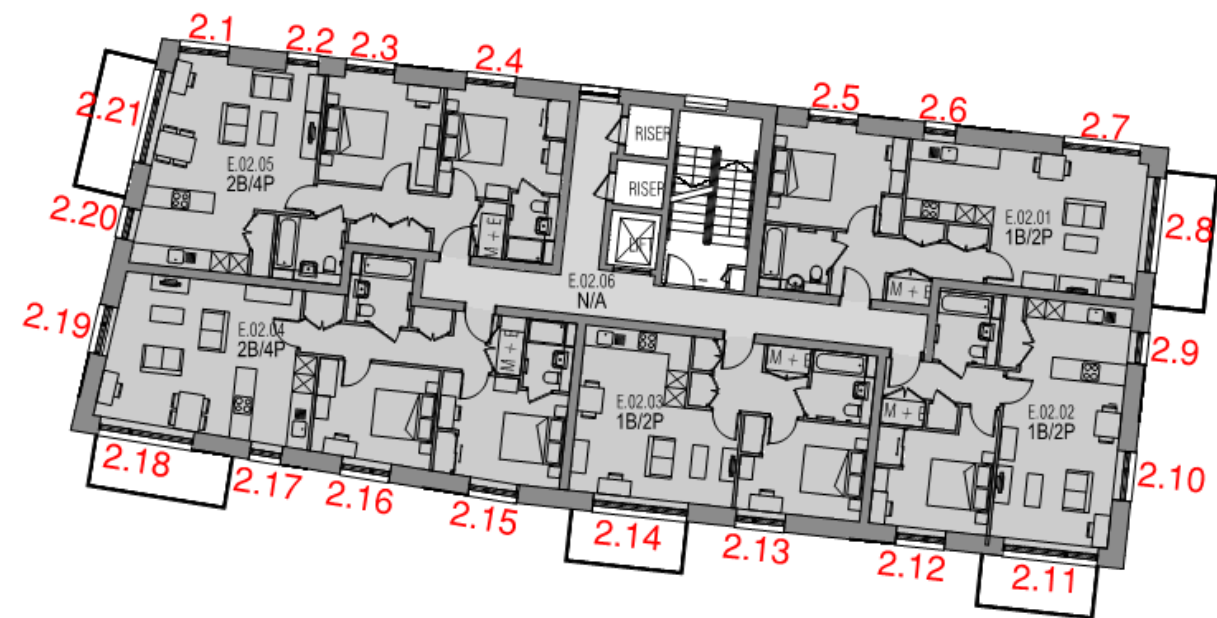
Figure 9 Building 303 Block E – Level 2 floor plan
