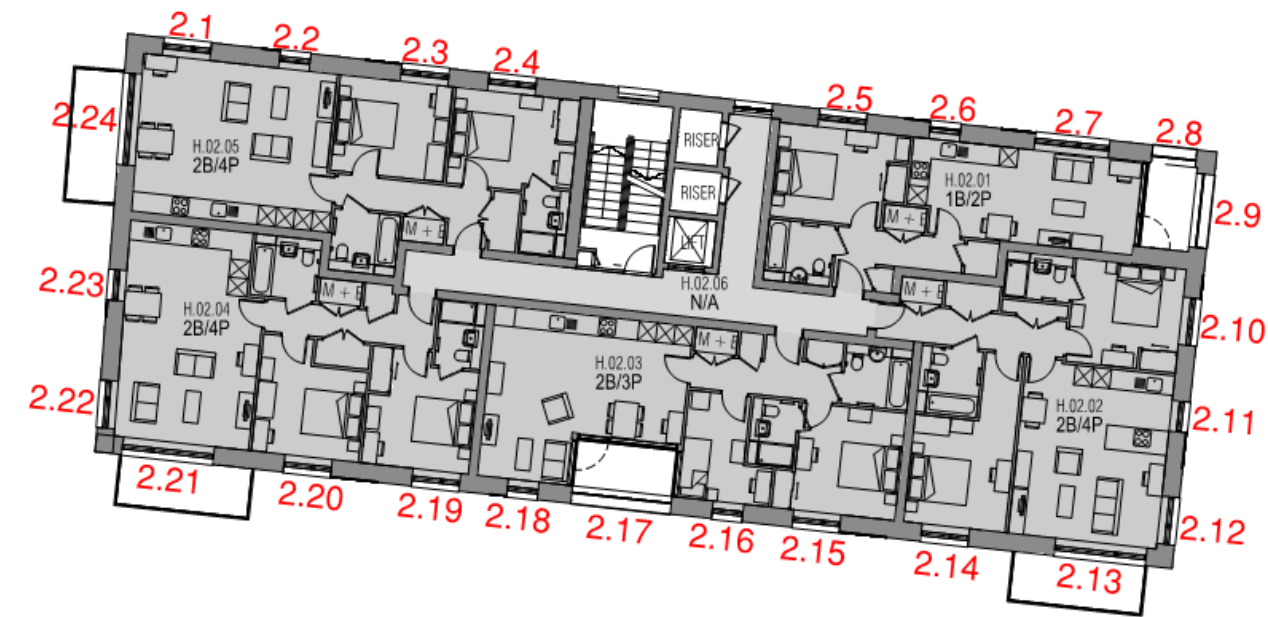
Figure 11 Building 303 Block H – Level 2 floor plan
