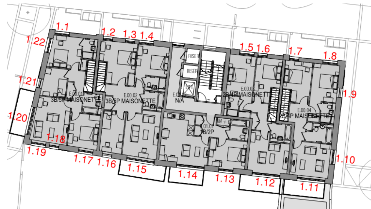
Figure 5 Building 303 Block E – Level 1 floor plan
