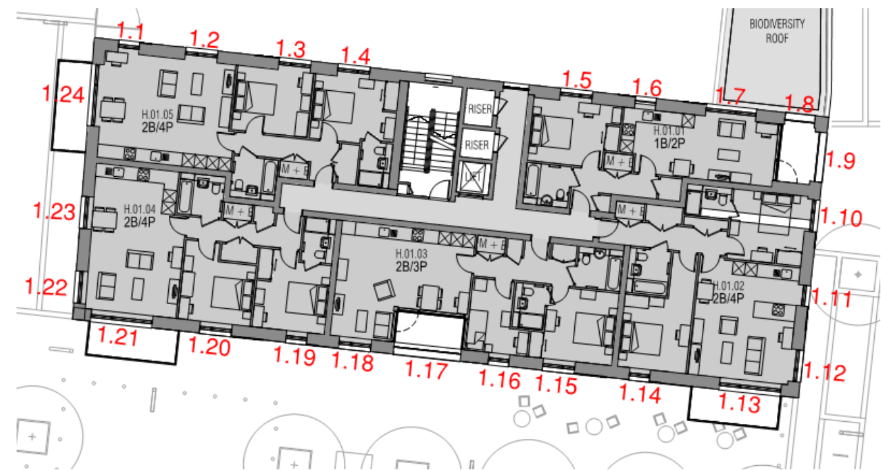
Figure 8 Building 303 Block H – Level 1 floor plan
