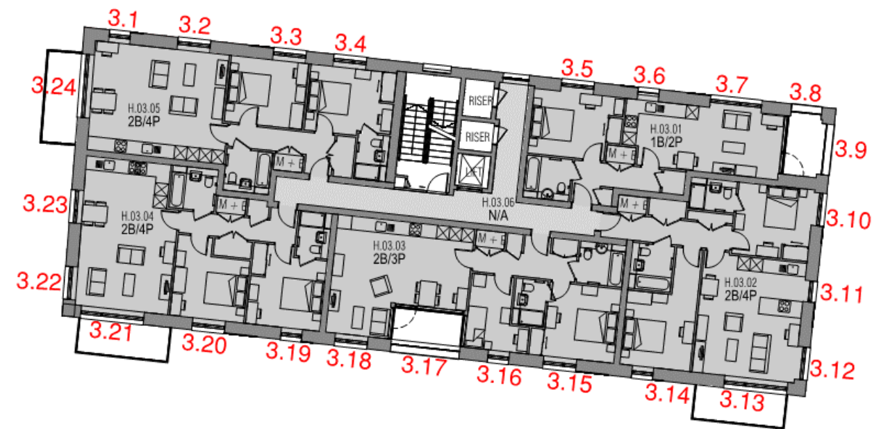
Figure 14 Building 303 Block H– Level 3 floor plan
