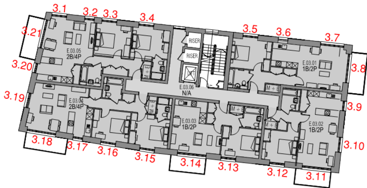
Figure 12 Building 303 Block E – Level 3 floor plan
