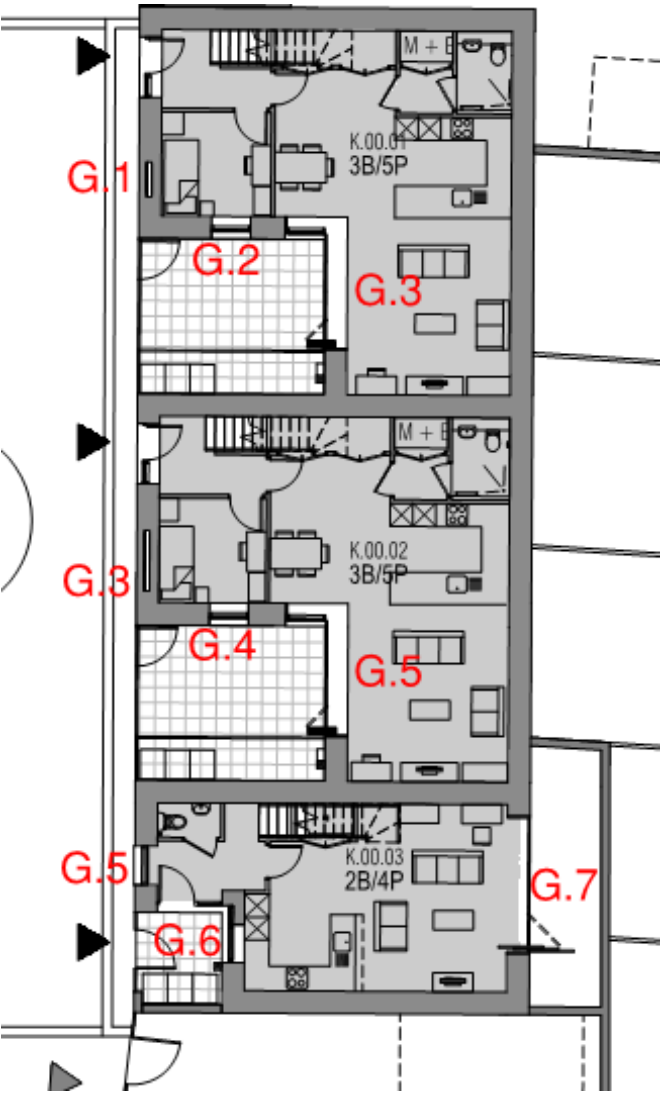
Figure 2 Building 304 Block K– Ground level floor plan
