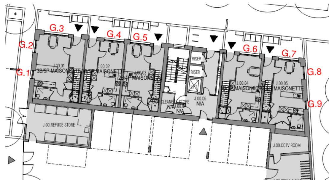
Figure 1 Building 304 Block J– Ground level floor plan
