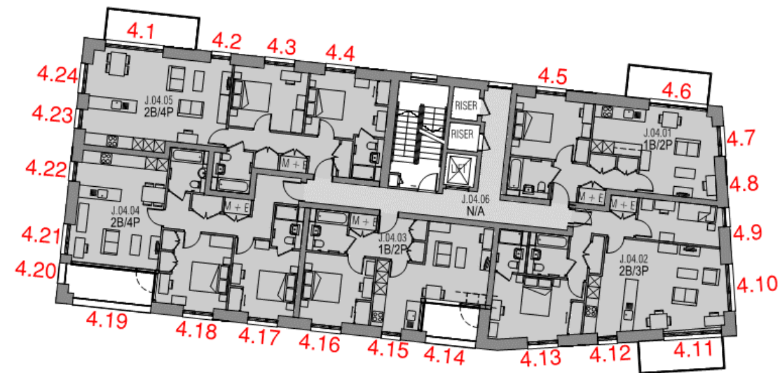
16 Building 304 Block J– Level 4
