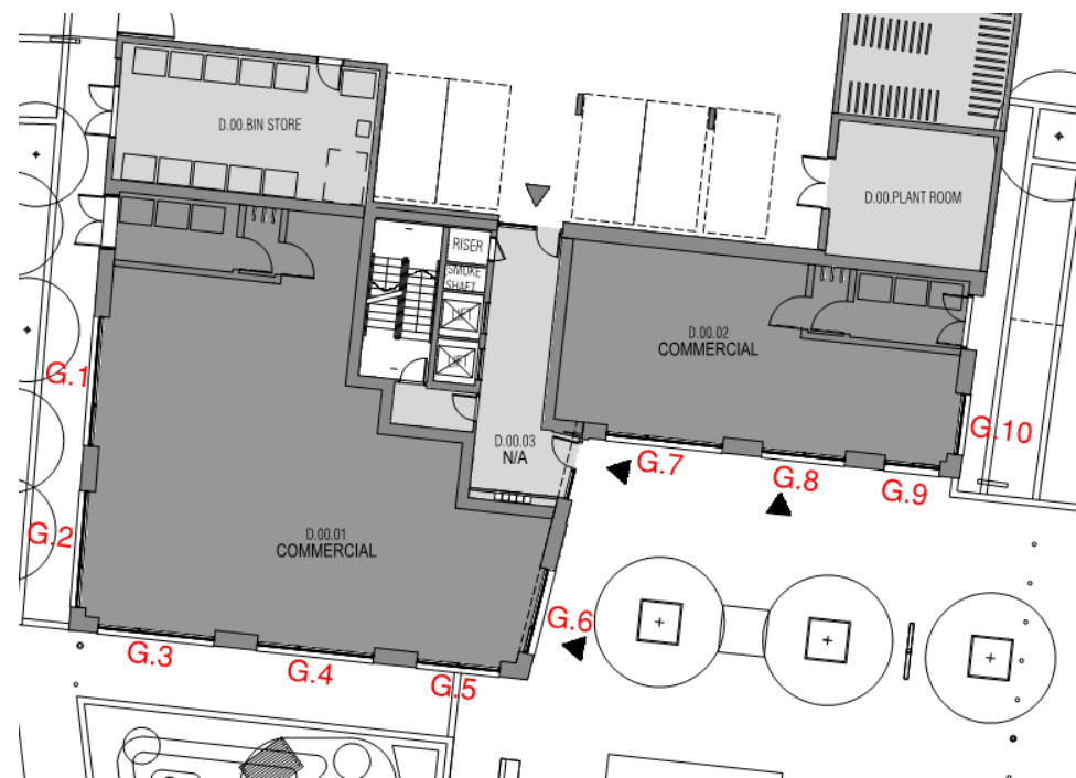
Figure 4 Building 302 Block D – Ground level floor plan
