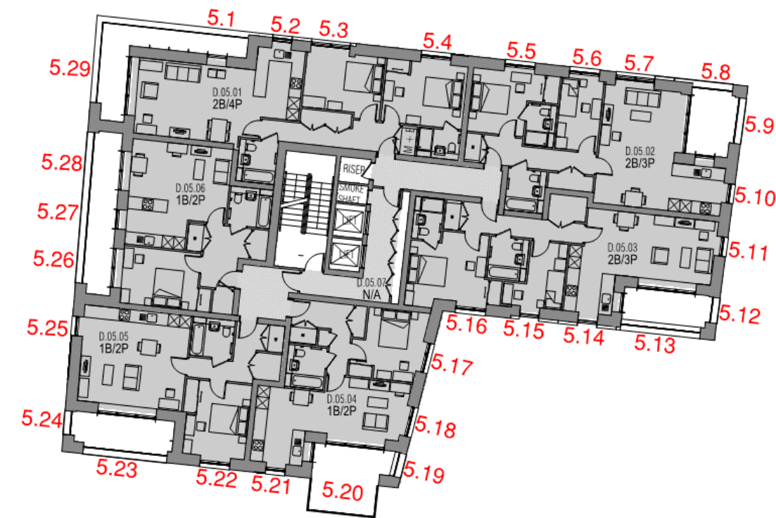
Figure 18 Building 302 Block D – Level 5 floor plan
