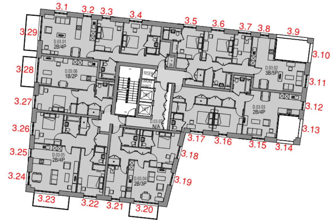
Figure 14 Building 302 Block D – Level 3 floor plan
