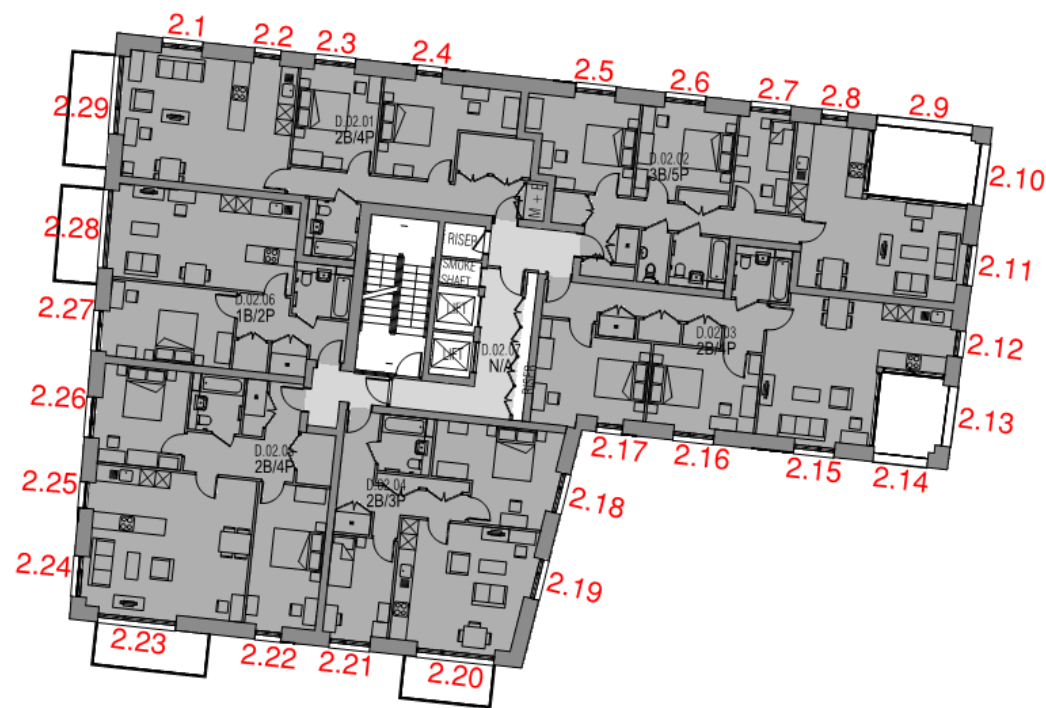
Figure 11 Building 302 Block D – Level 2 floor plan
