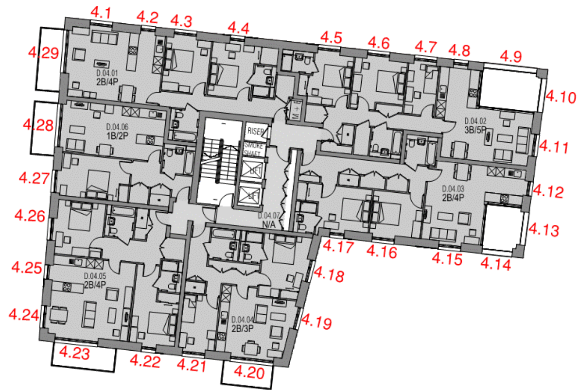
16 Building 302 Block D – Level 4
