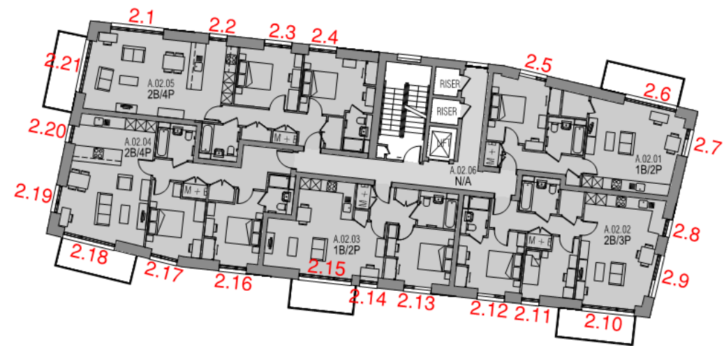
Figure 9 Building 302 Block A – Level 2 floor plan
