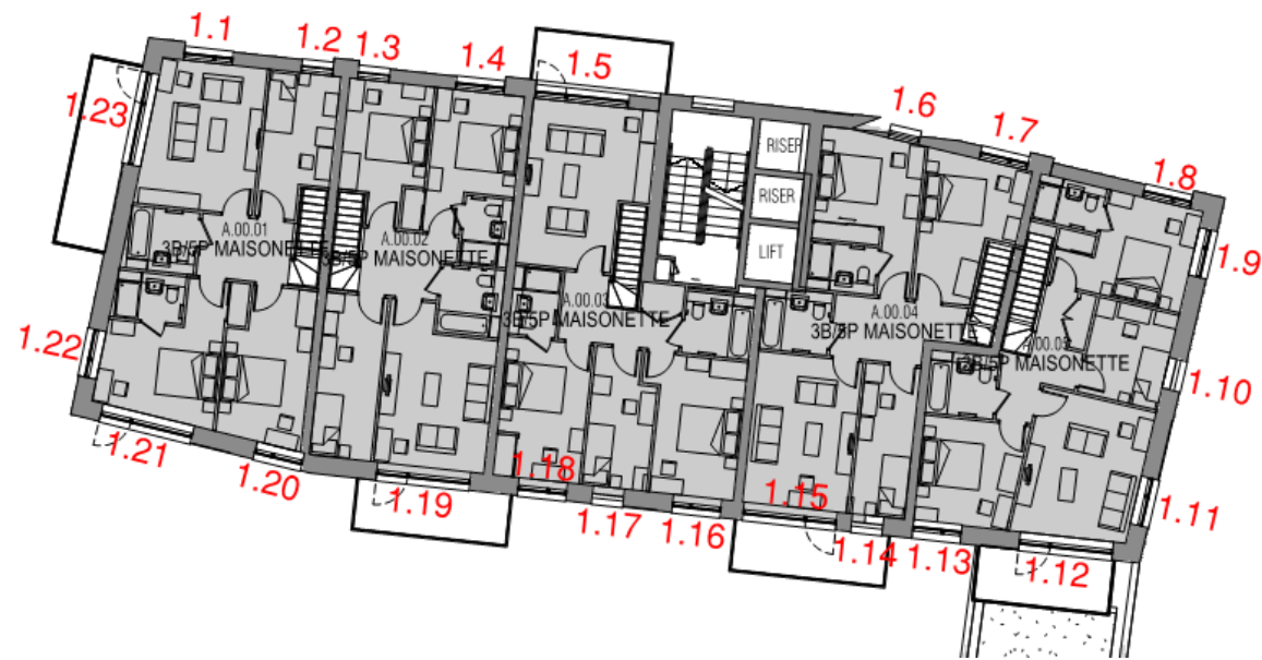
Figure 5 Building 302 Block A – Level 1 floor plan
