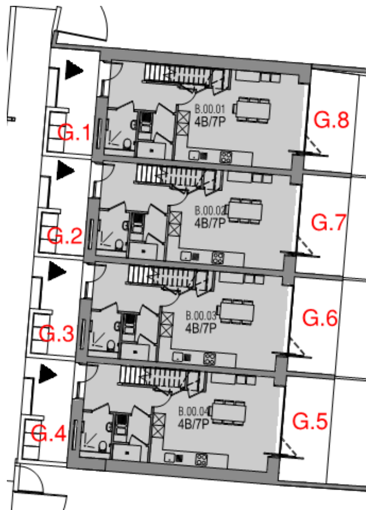
Figure 2 Building 302 Block B – Ground level floor plan
