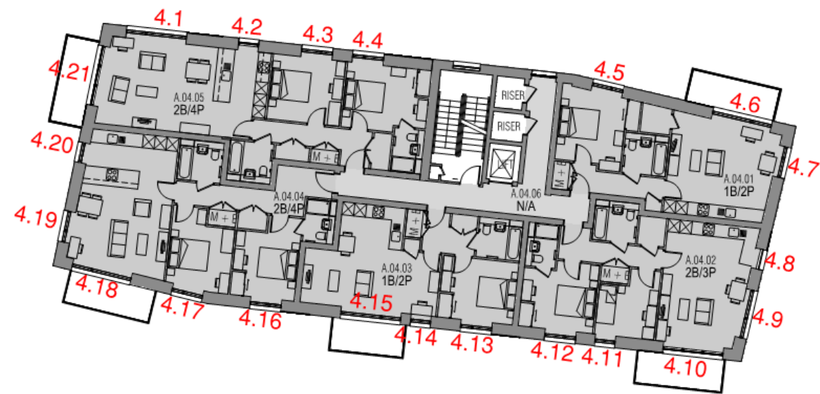
Figure 15 Building 302 Block A – Level 4 floor plan
