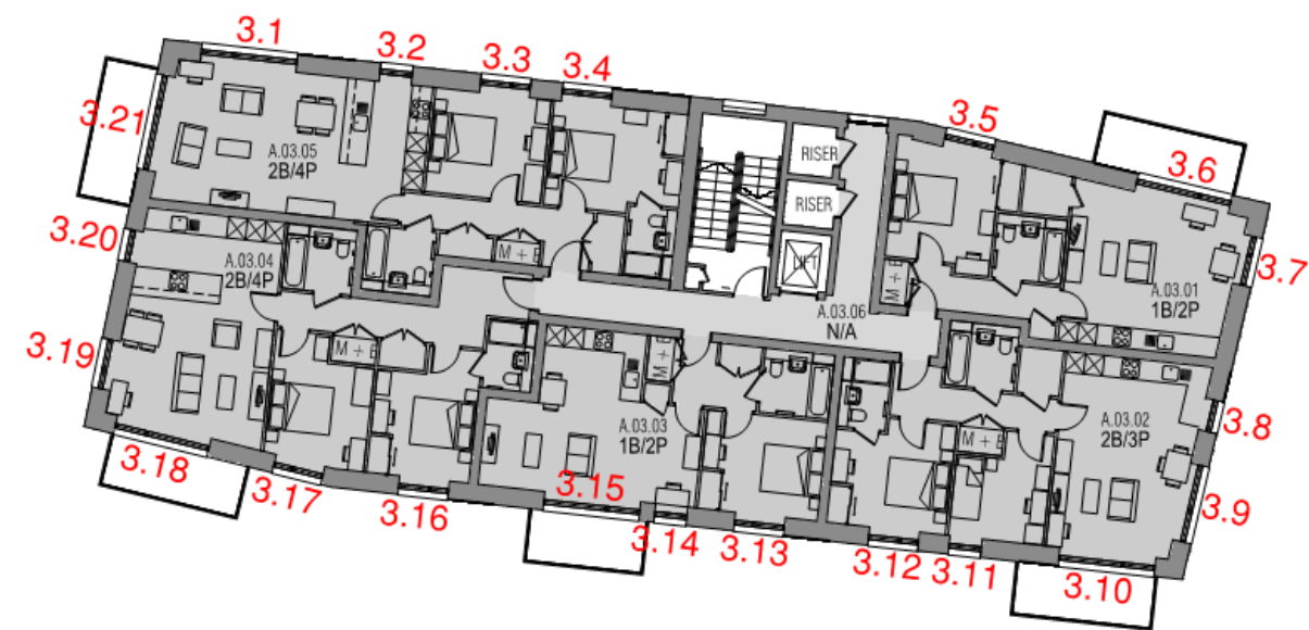
Figure 12 Building 302 Block A – Level 3 floor plan
