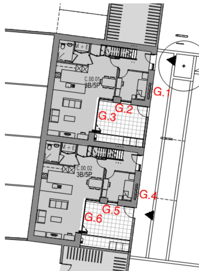
Figure 3 Building 302 Block C – Ground level floor plan
